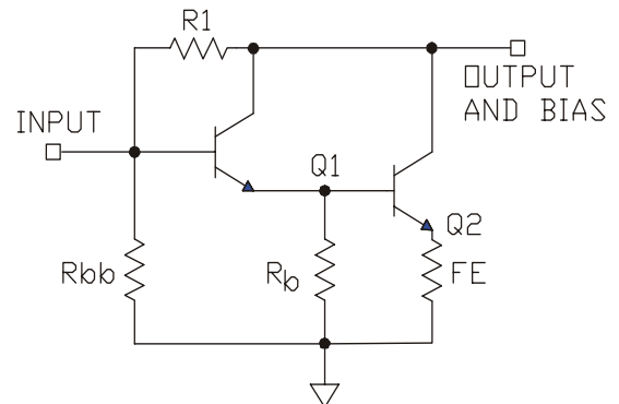
Simplified Schematic of MMIC
