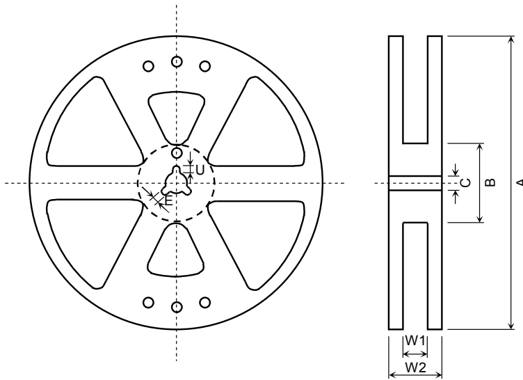
Figure 3 Reel Forms
