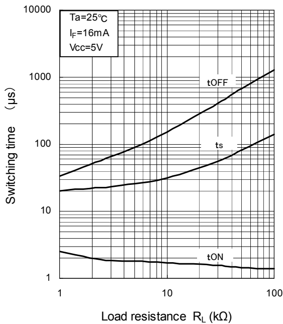
Switchingtime - R_L
