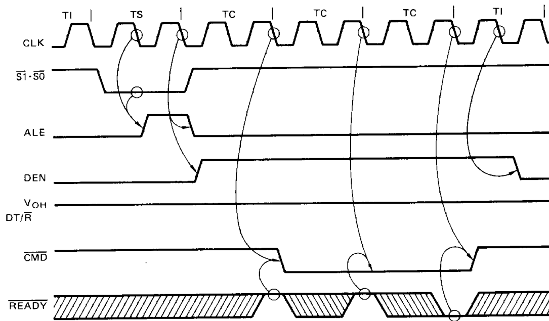
Fig. 10 – IDEL-WRITE-IDLE BUS CYCLES WITH MB = 1
