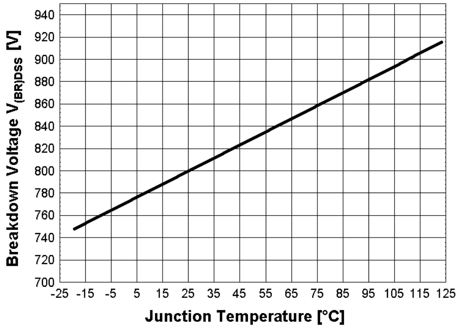
Figure 9 Drain-Source Breakdown voltage; V_{BR(DSS)} = f(T_j), I_D = 0.25mA
