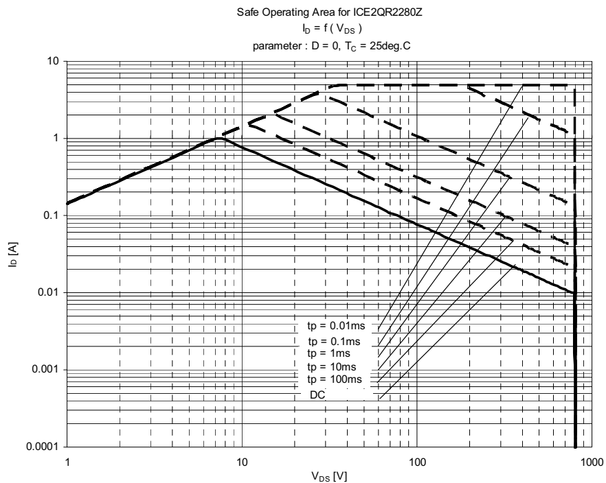
Figure 10 Safe Operating Area(SOA) for ICE2QR2280Z
