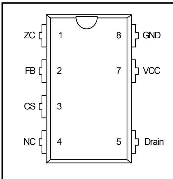
Figure 1 Pin Configuration PG-DIP7 (top view)
