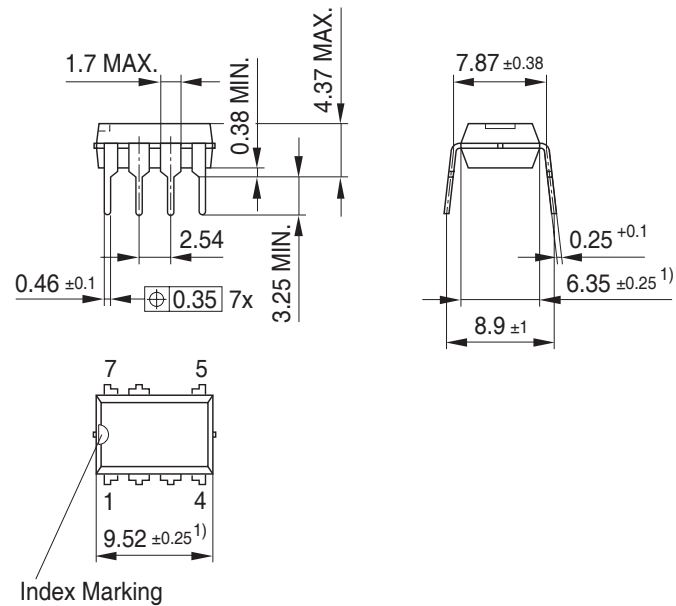
Figure 13 PG-DIP-7(Pb-free lead plating Plastic Dual In-Line Outline)
