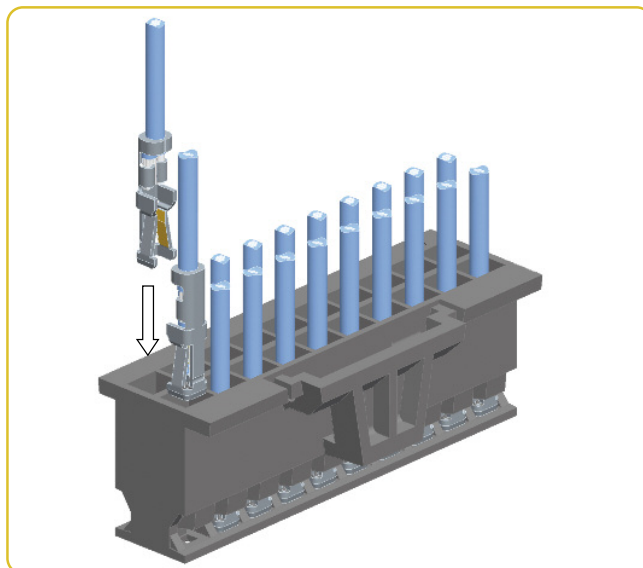
Insert the terminals into the active latch housing.
