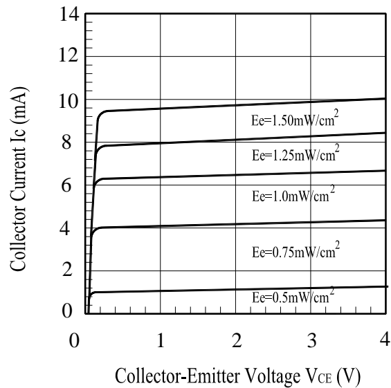
Fig.4 Collector Current vs. Collector-Emitter Voltage
