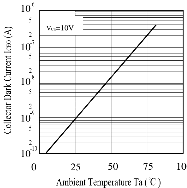
Fig.3. Collector Dark Current vs. Ambient Temperature
