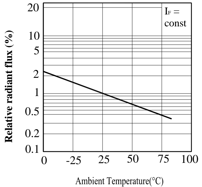
Fig.6 Relative Radiant Flux vs. Ambient Temperature(°C)
