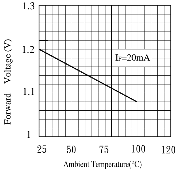
Fig.5 Forward Voltage vs. Ambient Temperature(°C)
