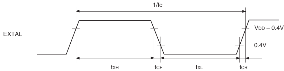
Fig. 1. Clock timing
