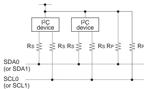
Fig. 9. I 2 C device recommended circuit
