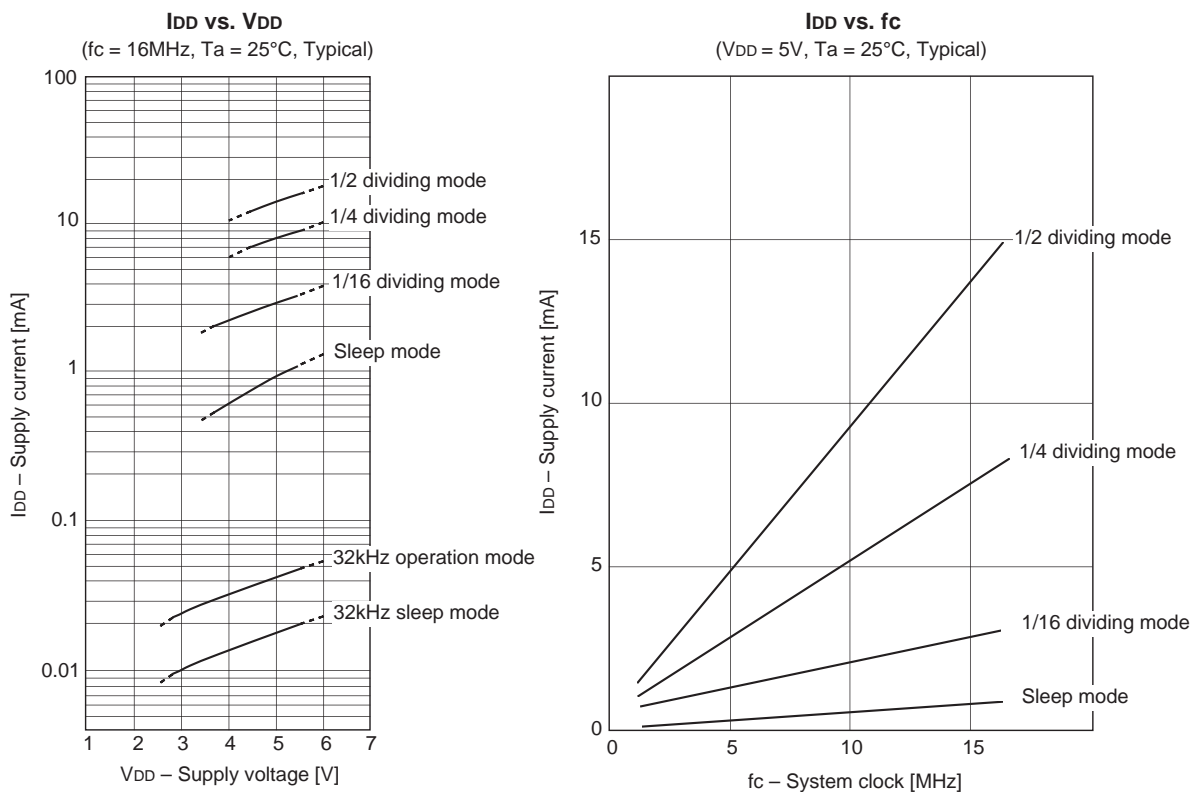
Fig. 11. Characteristic curves
