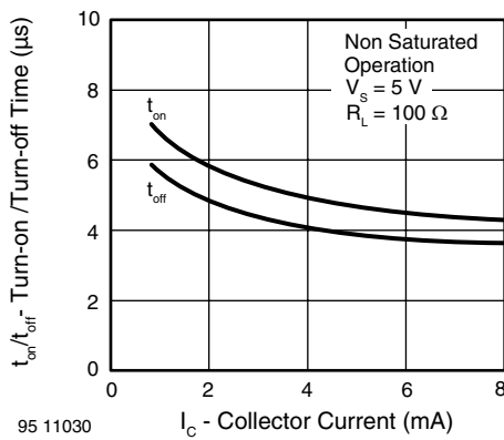
Fig. 13 - Turn-on/off Time vs. Collector Current
