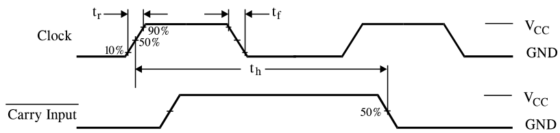
Figure 2. Switching Waveforms
