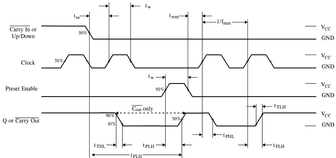
Figure 1. Switching Waveforms
