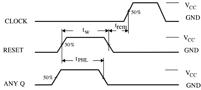
Figure 3. Switching Waveforms
