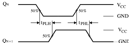
Figure 2. Switching Waveforms
