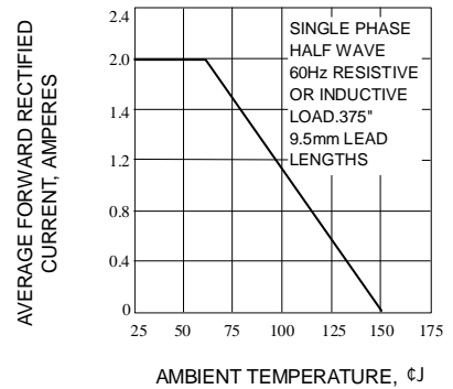
Fig. 2-MAXIMUM AVERAGE FORWARD CURRENT RATING
