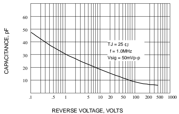
Fig. 6-TYPICAL JUNCTION CAPACITANCE
