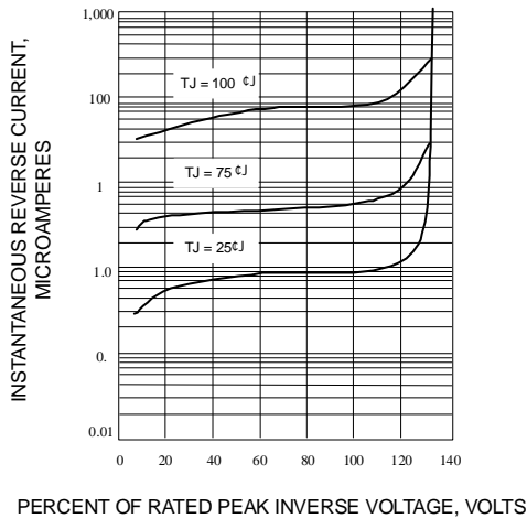
Fig. 3-TYPICAL REVERSE CHARACTERISTICS
