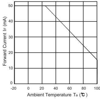
Forward Current vs. Ambient Temperature
