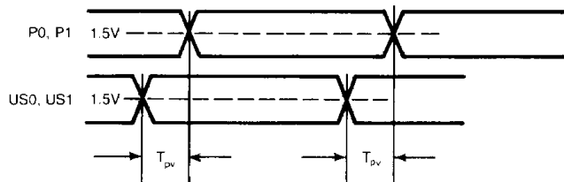
FIGURE 2: PRECOMP VALUE TIMING
