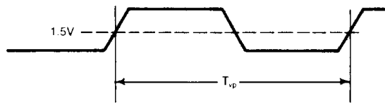
FIGURE 1: VCOCLK TIMING
