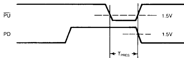
FIGURE 4: PUMPDOWN TO PUMPUP TIMING
