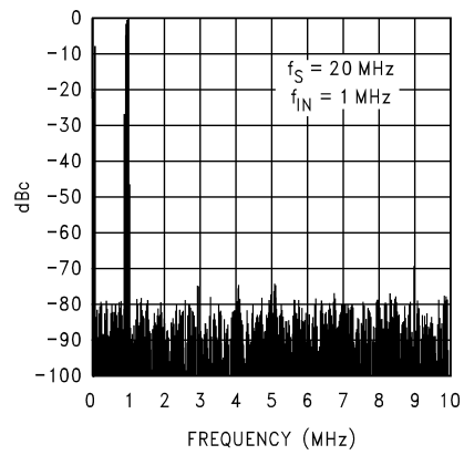
Spectral Response @ f_{IN} = 1\text{ MHz}
