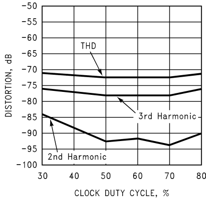
Distortion vs. Clock Duty Cycle @ f_{IN} = 4.7\text{ MHz}
