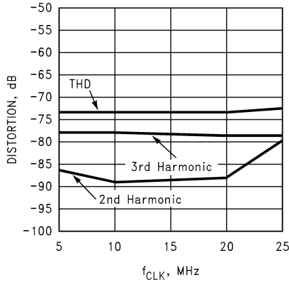
Distortion vs. f_{CLK} @ f_{IN} = 9.5\text{ MHz}
