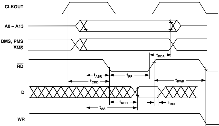
Figure 42. Memory Read
