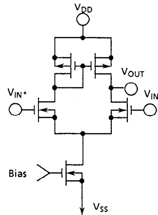
Figutr 18 Comparator
