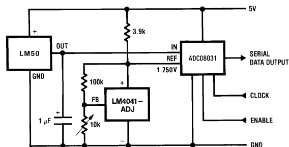
FIGURE 7. Temperature To Digital Converter (Serial Output) (+125 ^{\circ}\text{C} Full Scale)
