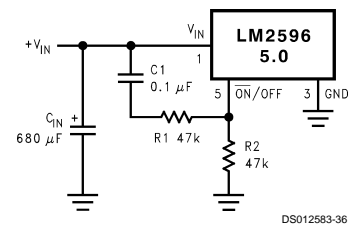
FIGURE 21. Delayed Startup
