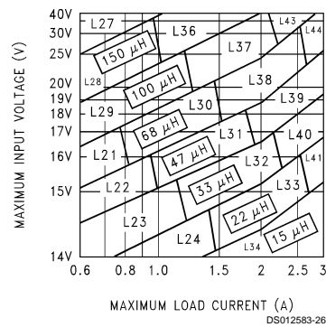
FIGURE 6. LM2596-12
