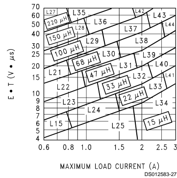
FIGURE 7. LM2596-ADJ
