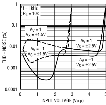
Total Harmonic Distortion + Noise vs Peak-to-Peak Voltage
