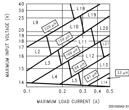
FIGURE 6. LM2671-12
