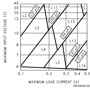
FIGURE 4. LM2671-3.3
