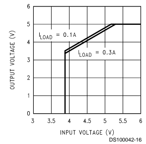
Dropout Voltage—5.0V Option
