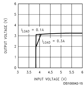
Dropout Voltage—3.3V Option
