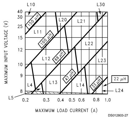
FIGURE 5. LM2675-5.0
