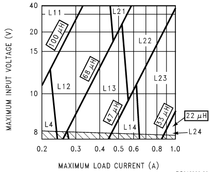
FIGURE 4. LM2675-3.3
