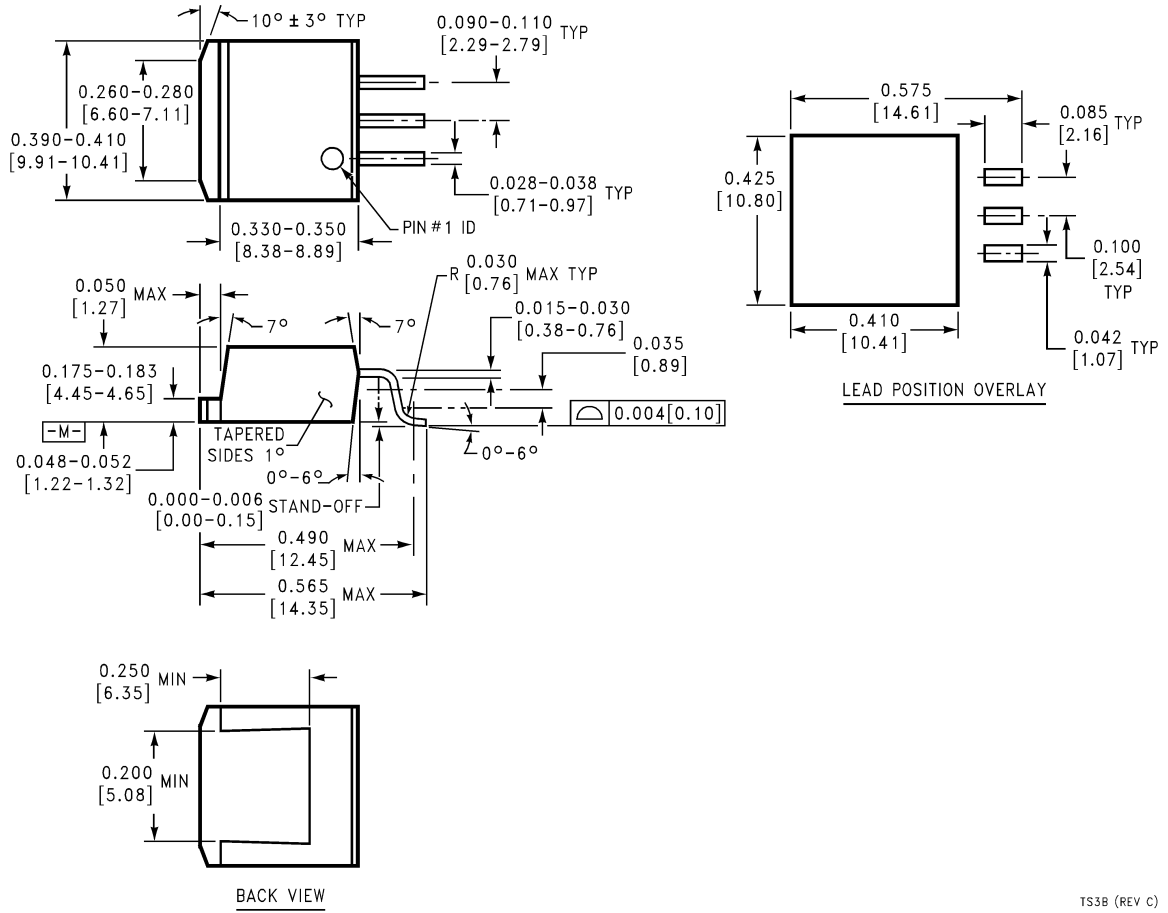
TO-263 3-Lead Plastic Surface Mount Package Order Number LM2937ES-5.0, LM2937ES-8.0, LM2937ES-10, LM2937ES-12 or LM2937ES-15 NS Package Number TS3B
