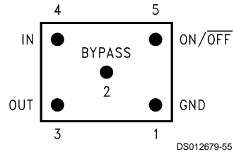
micro SMD, 5 Bump Package (BPA05)
