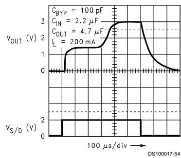
Turn-On Time (LP2988)
