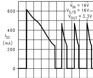
200 \text{ms}/\text{Div} DS100017-32
