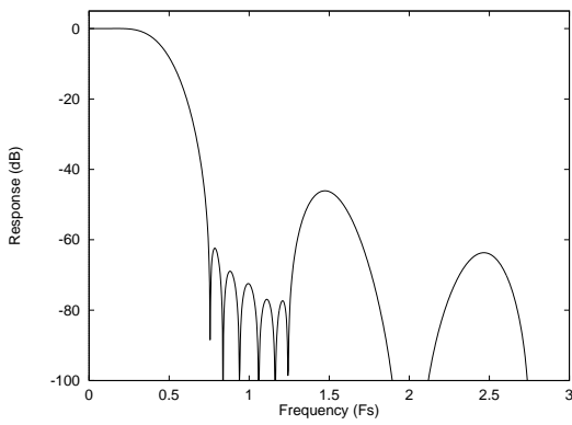
Figure 35 ADC Digital Filter Frequency Response – Type 2
