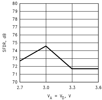
SFDR vs. Supply Voltage @ f_{IN} = 4.7 MHz
