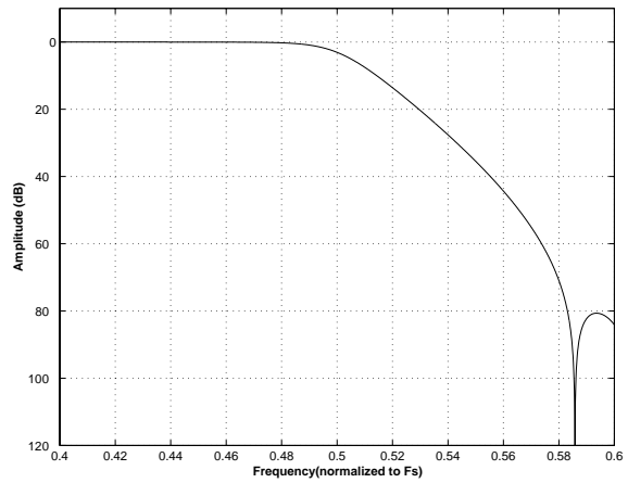
Figure 18. Double Speed (fast) Transition Band
