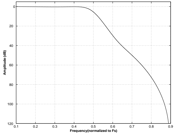
Figure 30. Quad Speed (slow) Transition Band
