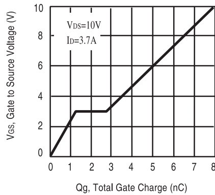
Figure 9. Gate Charge
