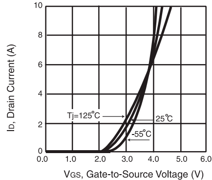
Figure 2. Transfer Characteristics
