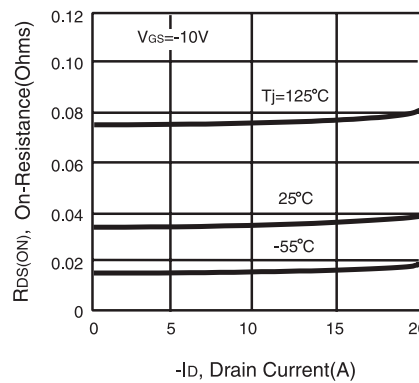
Figure 4. On-Resistance Variation with Drain Current and Temperature
