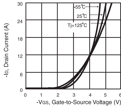
Figure 2. Transfer Characteristics
