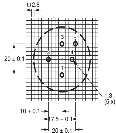
Case Ø D = 40 mm Fig.9 Mounting hole diagram viewed from component side
