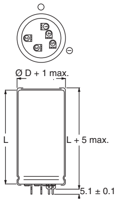
Case Ø D = 35 mm Fig.6 Printed wiring pin version
