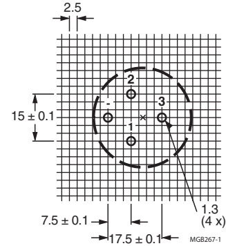
Case Ø D = 35 mm Fig. 7 Mounting hole diagram viewed from component side
