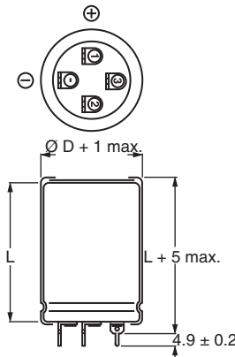
Case Ø D = 35 mm Fig.6 Printed wiring pin version
