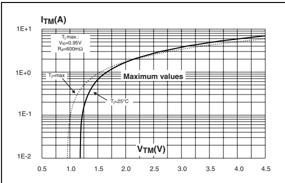
Figure 13. On-state characteristics P010xxA, P010xxN
