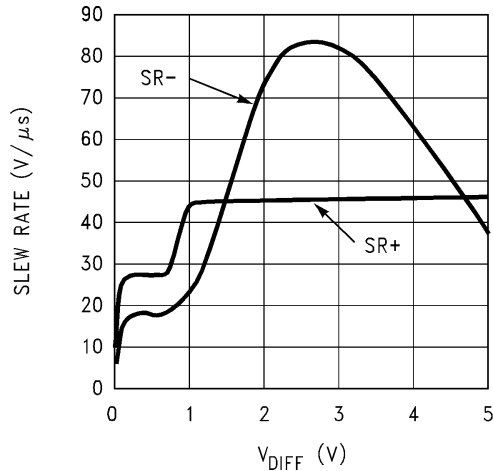
FIGURE 2. Slew Rate vs. V_{DIFF}
