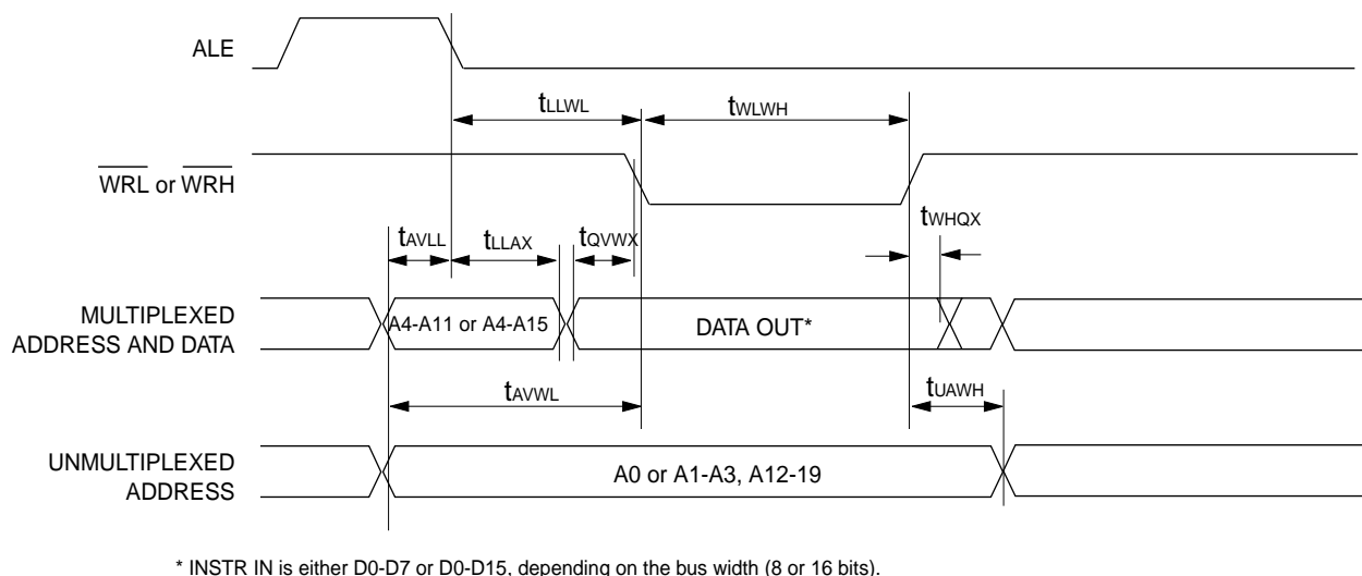
Figure 24. External Data Memory Write Cycle
