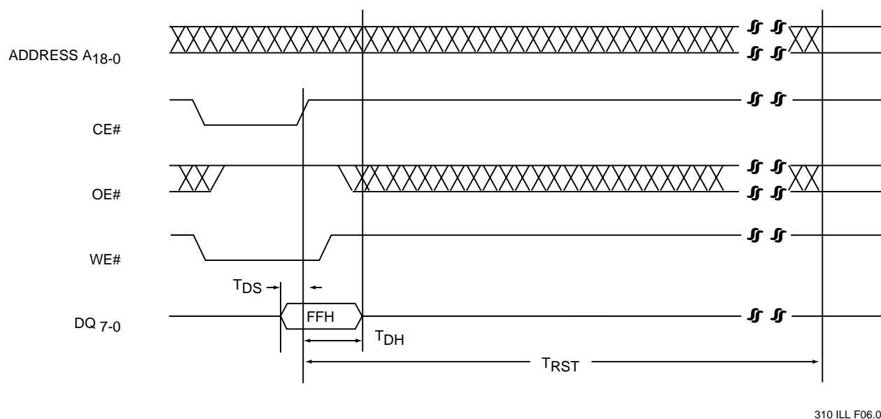
FIGURE 7: RESET COMMAND TIMING DIAGRAM
