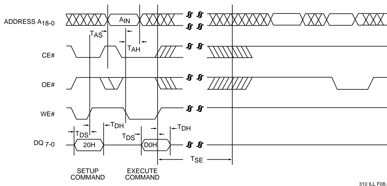
FIGURE 9: SECTOR-ERASE TIMING DIAGRAM
