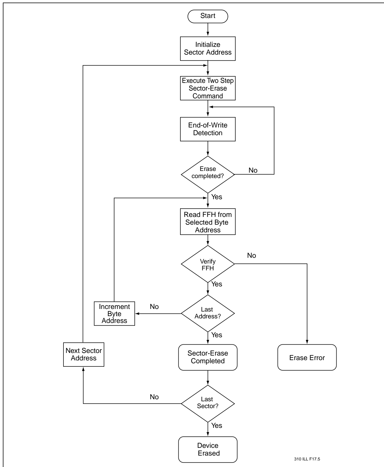
FIGURE 18: SECTOR-ERASE FLOWCHARTS
