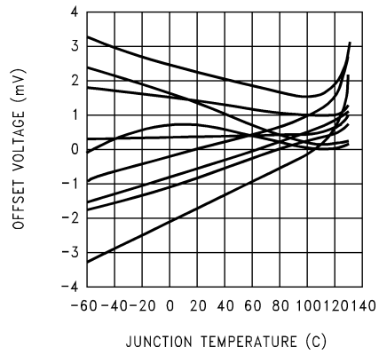
V_{OS} vs. Junction Temperature on 9 Representative Units
