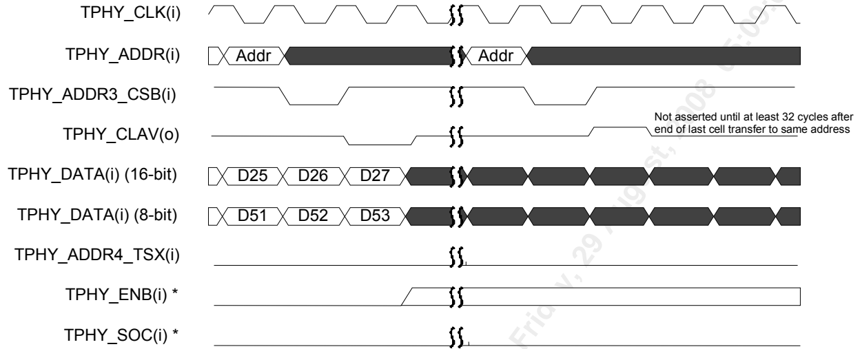
Figure 103 SNK_INTF End-of-Transfer (Any-PHY PHY Mode)
