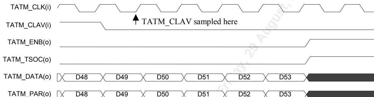
Figure 87 SRC_INTF End-of-Transfer Timing (Utopia 1 ATM Mode)
