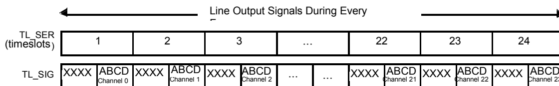
Figure 70 Output of T1 Signaling Bits
