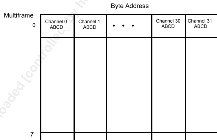
Figure 22 SDF-MF E1 Format of the T_SIGNALING_BUFFER
