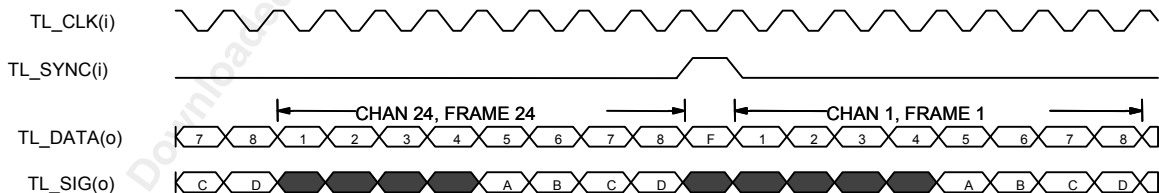
Figure 115 Transmit Line Side T1 Timing(TL_CLK = 1.544 MHz)
