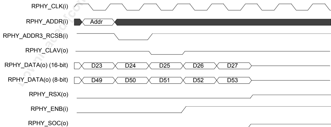
Figure 93 UI_SRC_INTF End-of-Transfer Timing (Any-PHY PHY mode)
