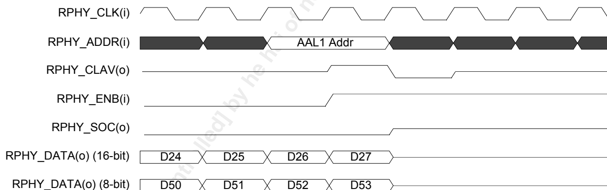
Figure 91 UI_SRC_INTF End-of-Transfer Timing (Utopia 2 PHY Mode)
