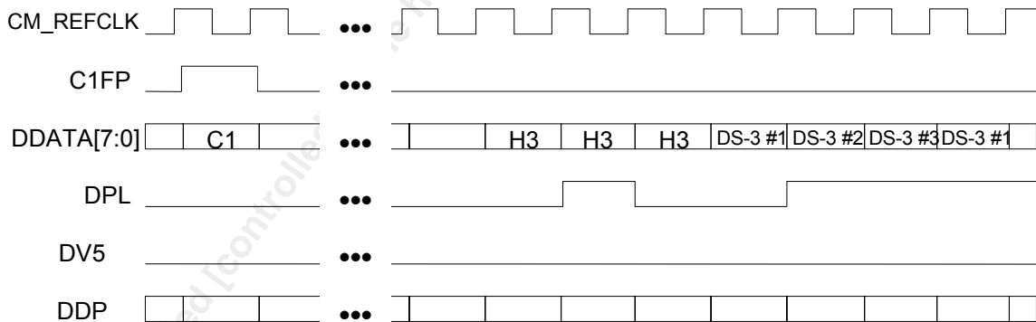
Figure 123 SBI DROP Bus DS3 Functional Timing
