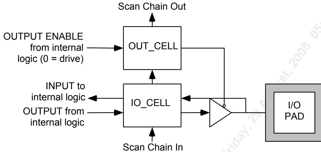
Figure 83 Layout of Output Enable and Bidirectional Cells
