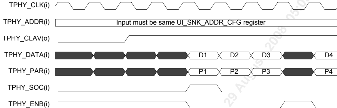
Figure 96 SNK_INTF Start-of-Transfer Timing (Utopia 1 PHY Mode)
