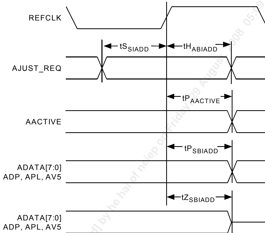
Figure 141 SBI ADD BUS Collision Avoidance Timing
