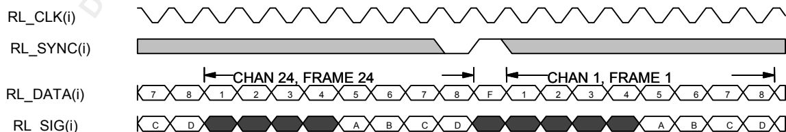
Figure 112 Receive Line Side T1 Timing(RL_CLK = 1.544 MHz)
