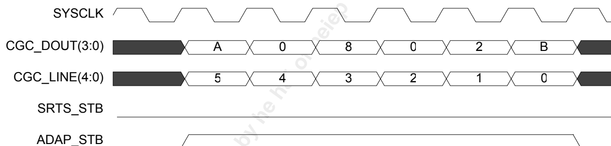
Figure 54 Adaptive Data Functional Timing
