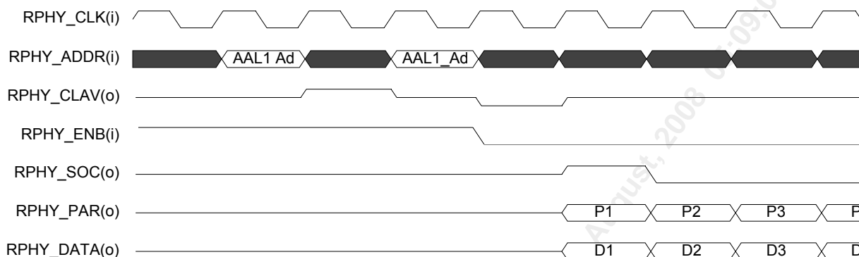
Figure 90 UI_SRC_INTF Start-of-Transfer Timing (Utopia 2 PHY Mode)
