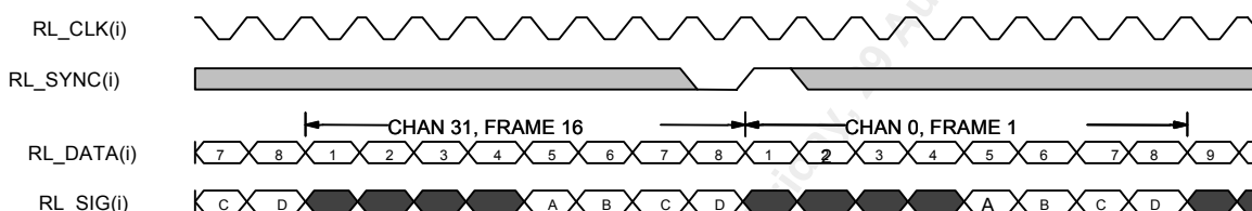
Figure 113 Receive Line Side E1 Timing(RL_CLK = 2.048 MHz)
