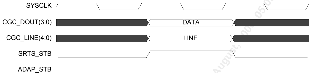
Figure 52 SRTS Data
