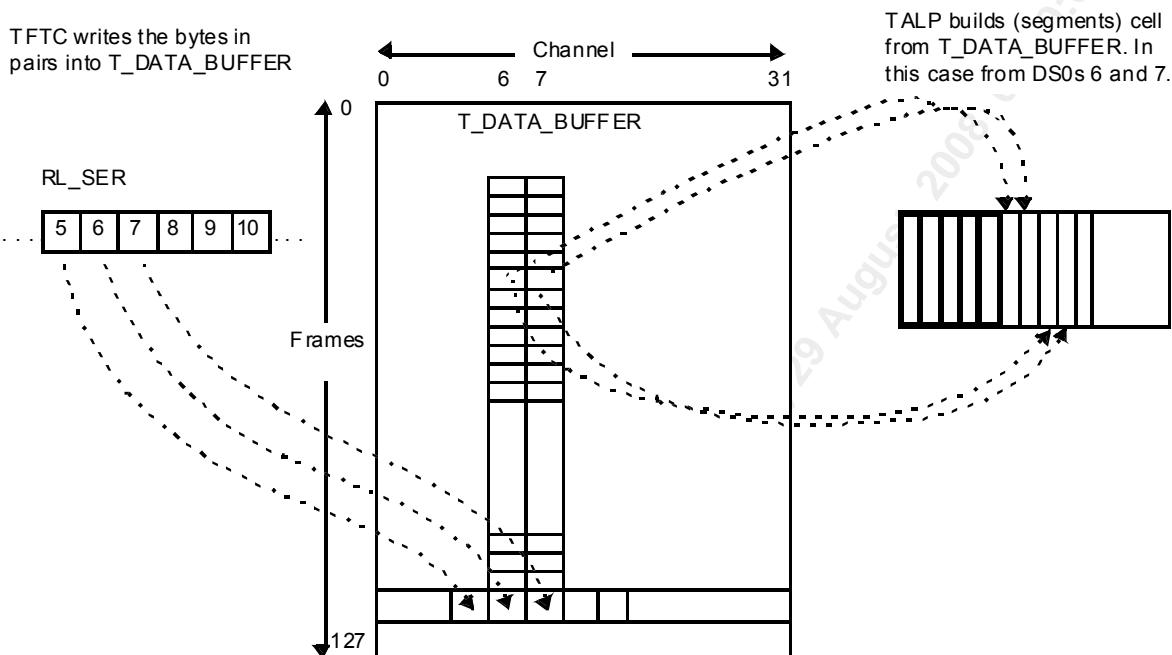
Figure 28 Payload Generation
