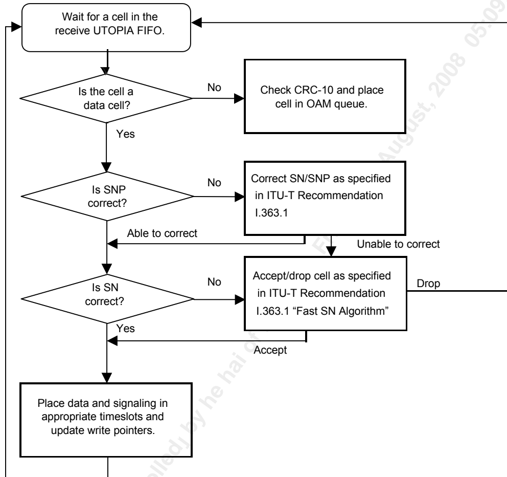
Figure 32 Receive Cell Processing for Fast SN
