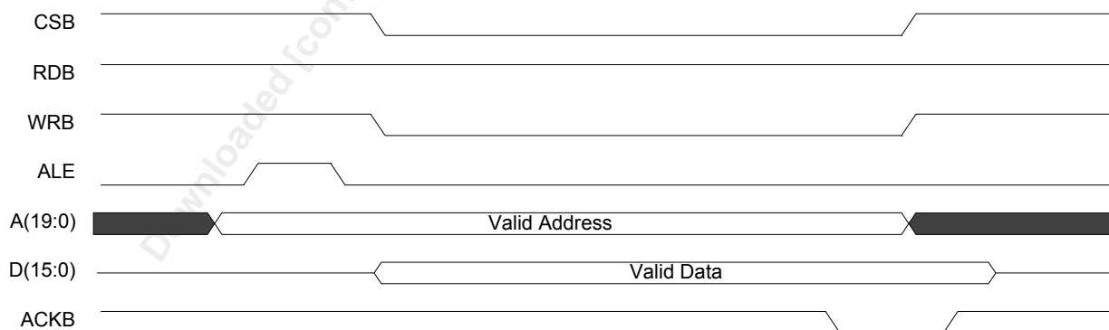
Figure 104 Microprocessor Write Access
