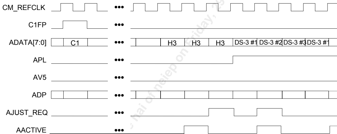
Figure 124 SBI ADD Bus Adjustment Request Functional Timing
