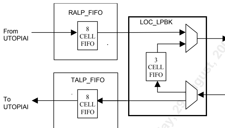
Figure 29 Local Loopback
