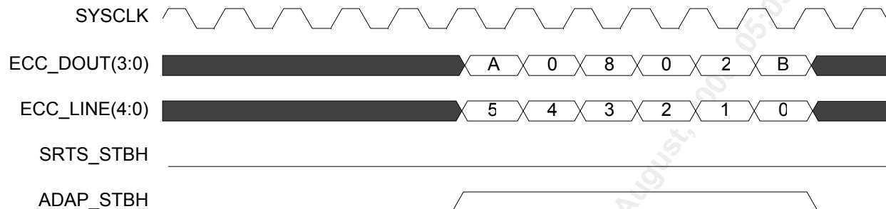
Figure 110 Adaptive Data Functional Timing
