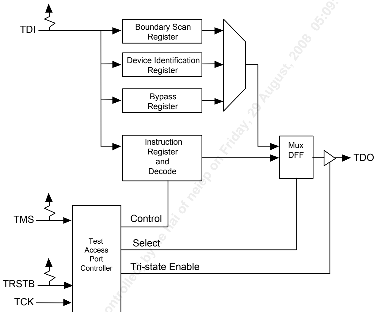
Figure 78 Boundary Scan Architecture
