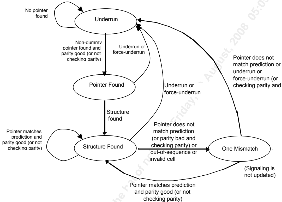
Figure 46 Pointer/Structure State Machine
