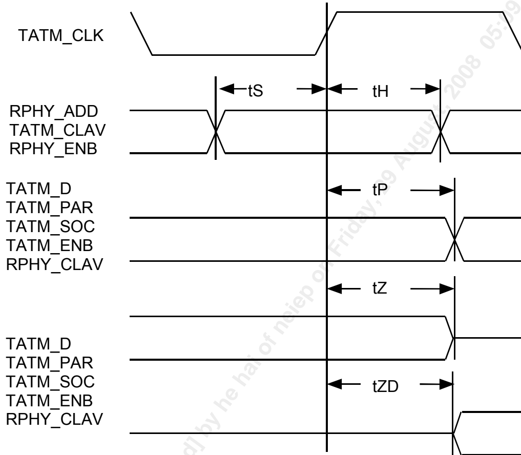
Figure 135 Source UTOPIA Interface Timing
