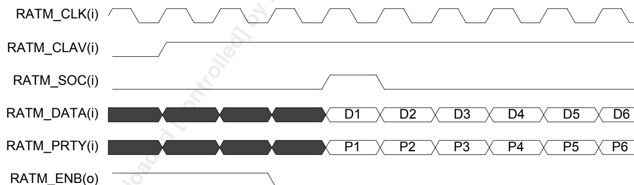
Figure 94 SNK_INTF Start-of-Transfer Timing (Utopia 1 ATM Mode)
