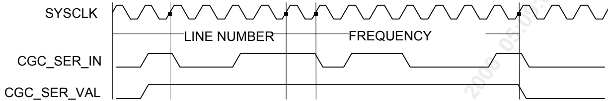
Figure 111 Ext Freq Select Functional Timing
