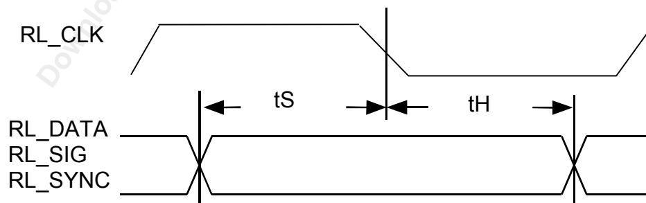
Figure 137 Receive Low Speed Interface Timing
