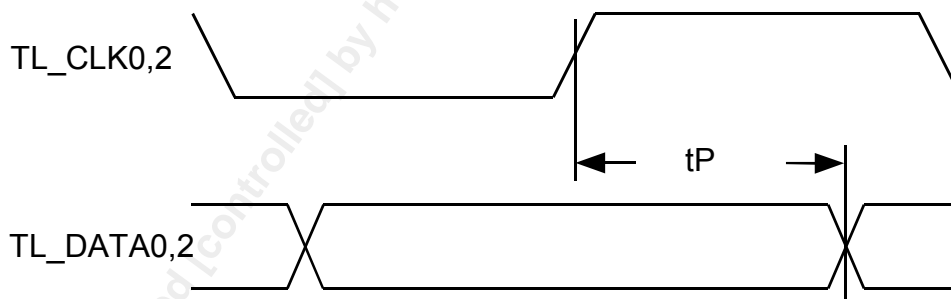
Figure 144 Transmit High Speed Timing
