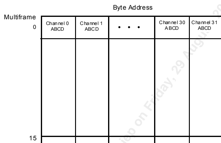
Figure 45 E1 SDF-MF with T1 Signaling Format of the R_SIG_BUFFER
