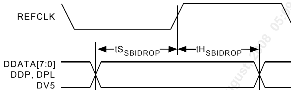
Figure 139 SBI DROP BUS Timing
