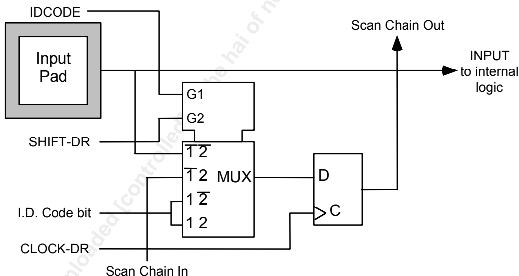
Figure 80 Input Observation Cell (IN_CELL)
