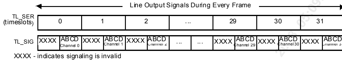
Figure 49 Output of E1 Signaling Bits (SHIFT_CAS=0)
