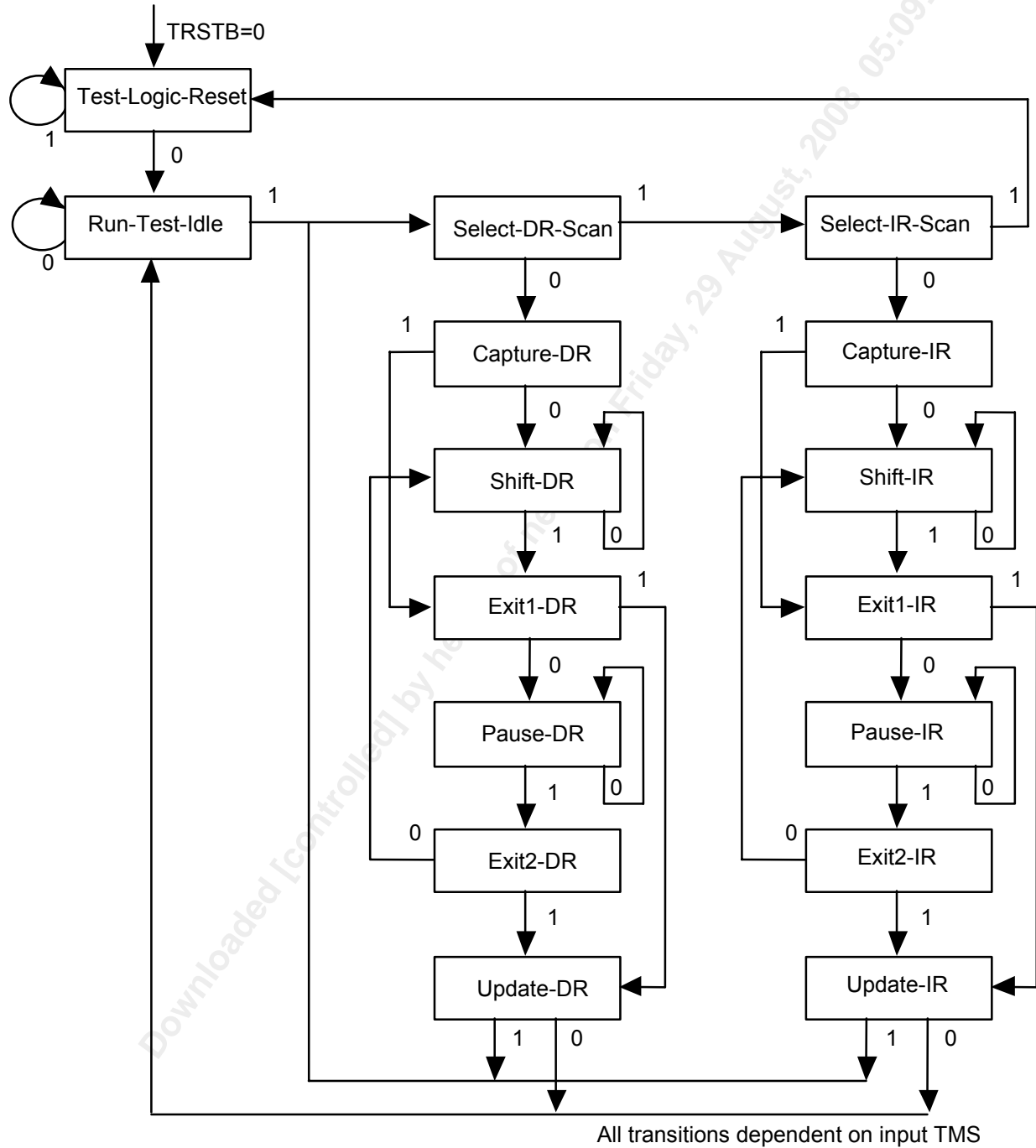
Figure 79 TAP Controller Finite State Machine
