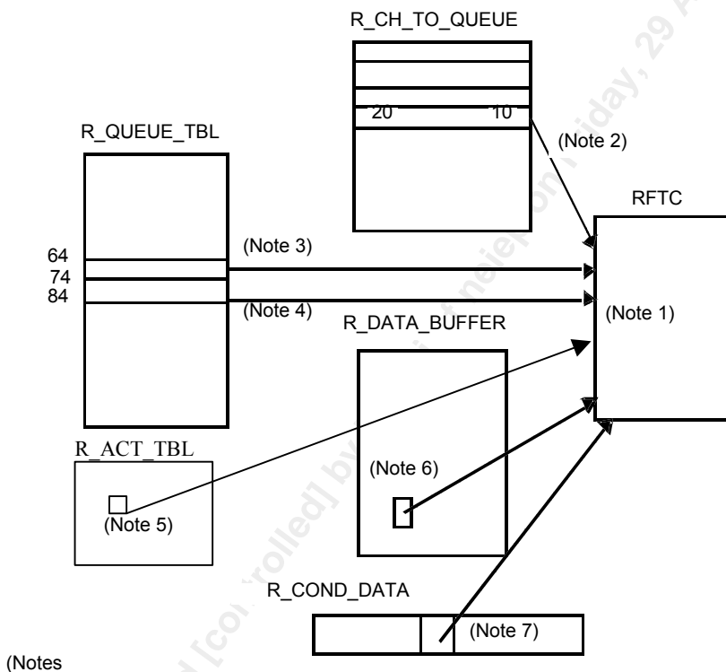
Figure 50 Channel-to-Queue Table Operation
