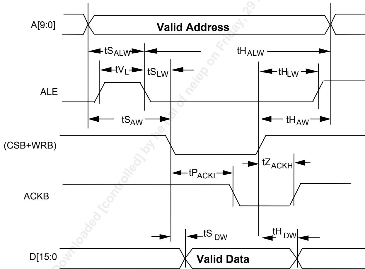
Figure 131 Microprocessor Interface Write Timing
