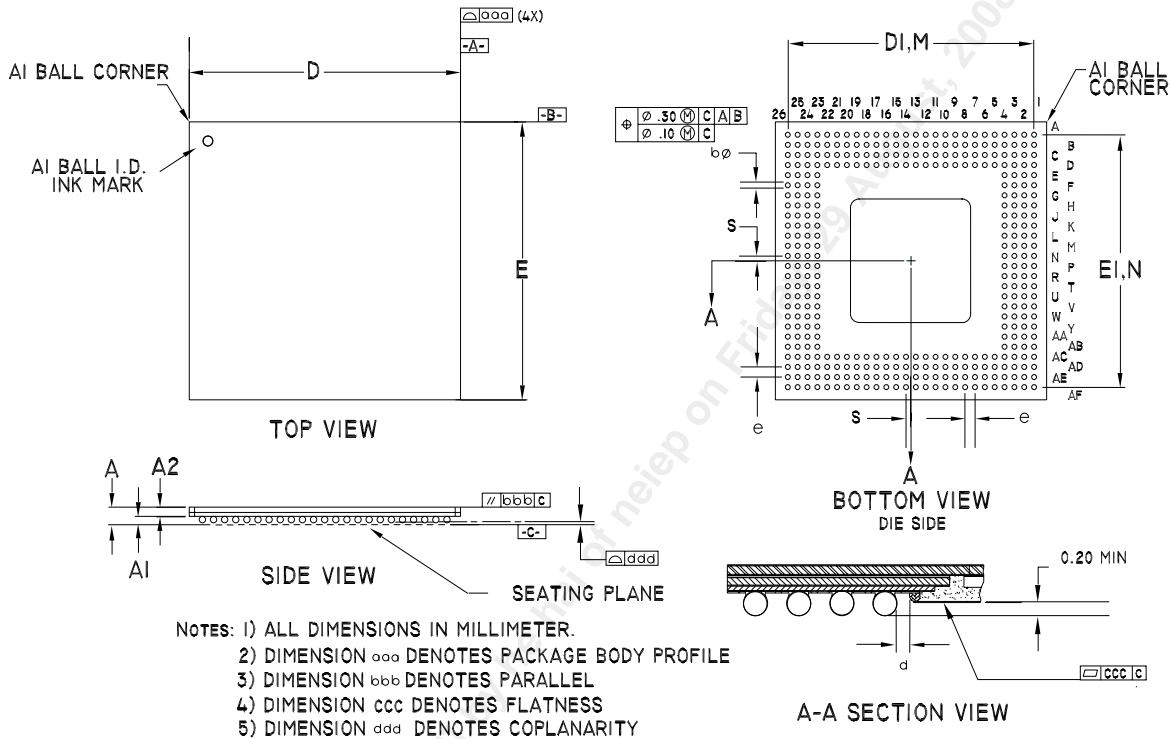
Figure 147 352 Pin Enhanced Ball Grid Array (SBGA)
