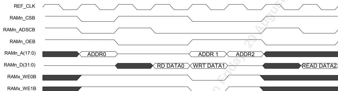
Figure 84 Pipelined Single-Cycle Deselect SSRAM
