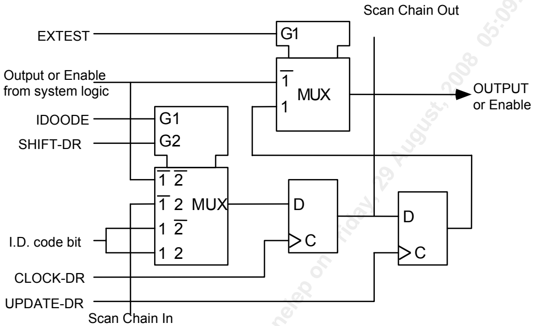
Figure 81 Output Cell (OUT_CELL)
