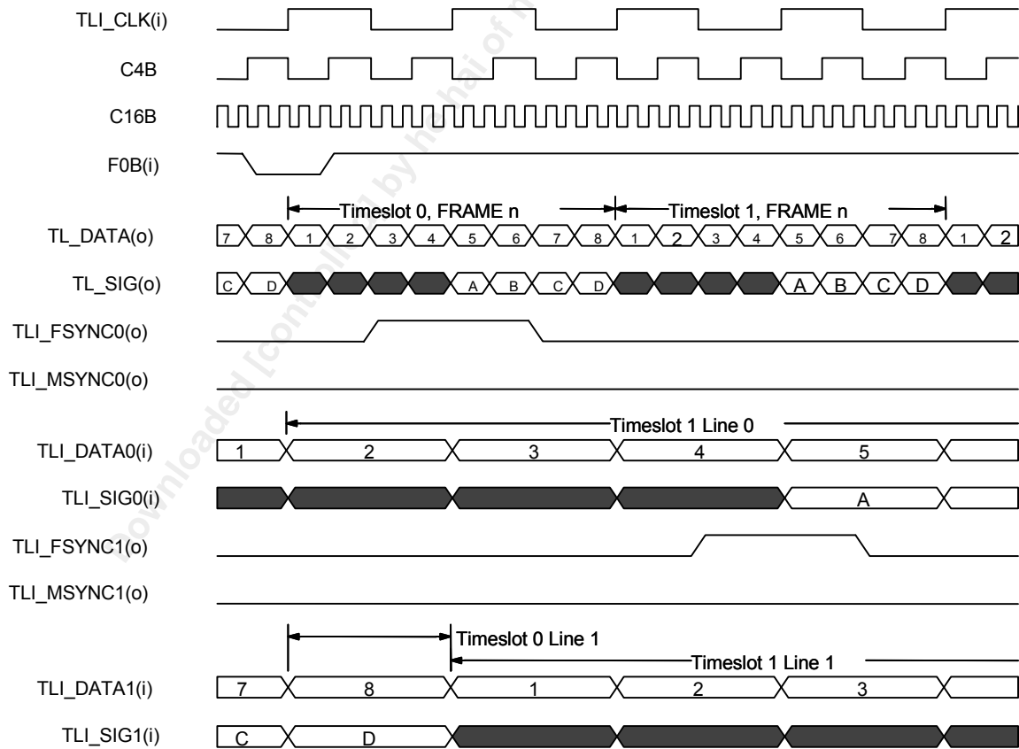
Figure 120 Transmit H-MVIP Timing, Close-up View
