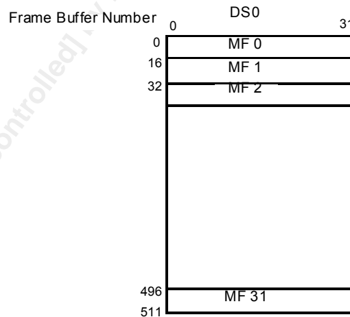
Figure 38 E1 SDF-MF Format of the R_DATA_BUFFER
