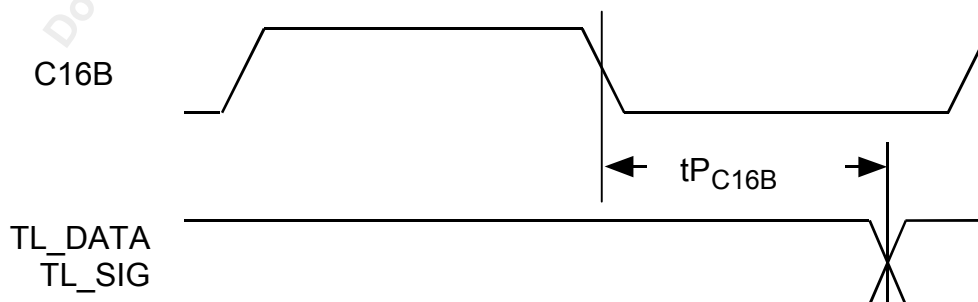
Figure 143 H-MVIP Ingress Data Timing
