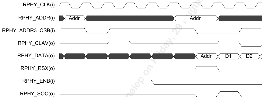
Figure 92 UI_SRC_INTF Start-of-Transfer Timing (Any-PHY PHY Mode)
