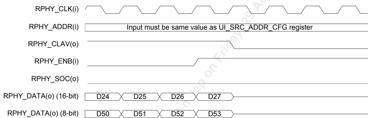
Figure 89 UI_SRC_INTF End-of-Transfer (Utopia 1 PHY Mode)
