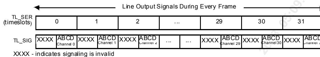
Figure 71 Output of E1 Signaling Bits
