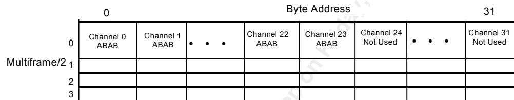
Figure 21 SDF-MF T1 SF Format of the T_SIGNALING_BUFFER
