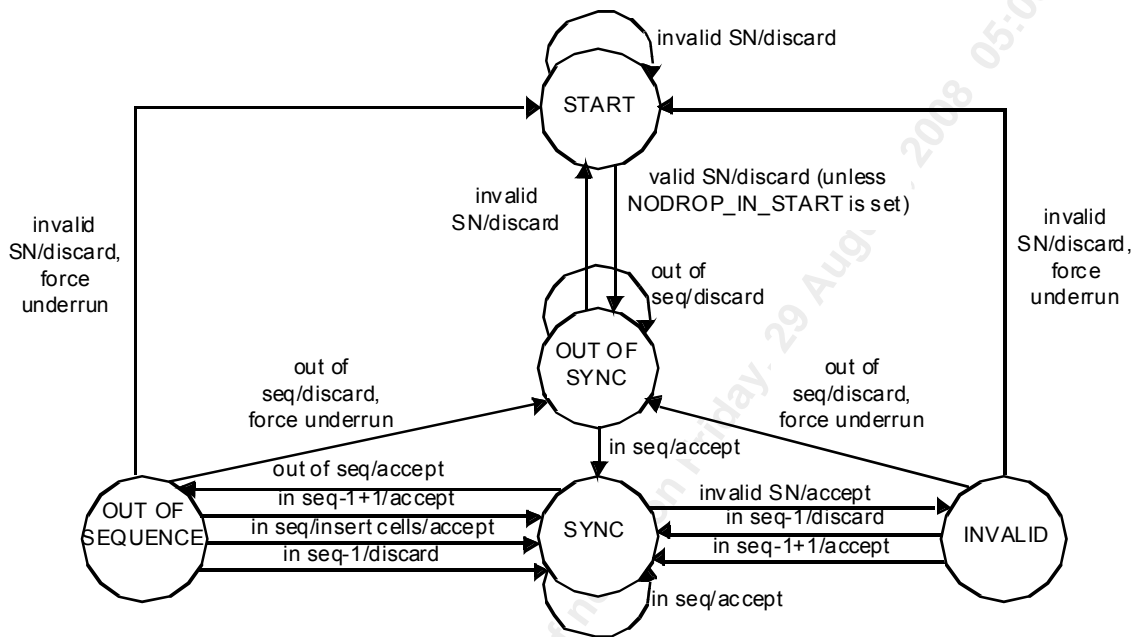
Figure 31 Fast SN Algorithm
