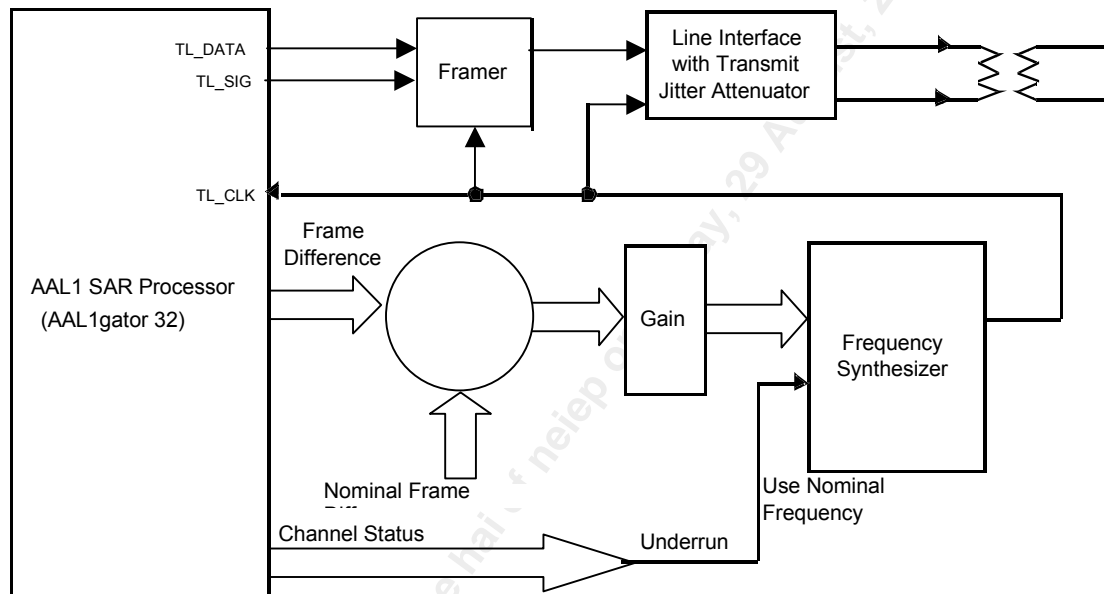
Figure 57 Direct Adaptive Clock Operation
