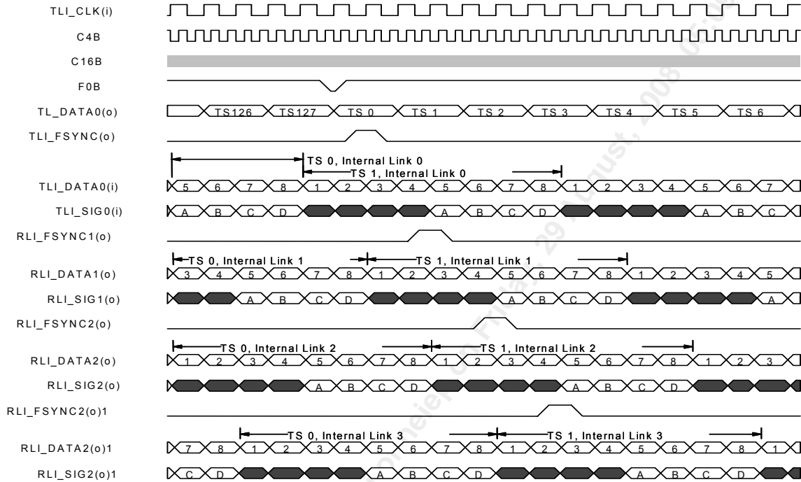
Figure 121 Transmit H-MVIP Timing, Expanded View
