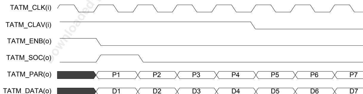
Figure 86 SRC_INTF Start of Transfer Timing (Utopia 1 ATM Mode)
