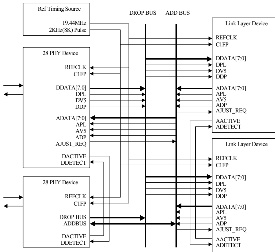
Figure 73 Multi-PHY to Multi-Link Layer Device Interface
