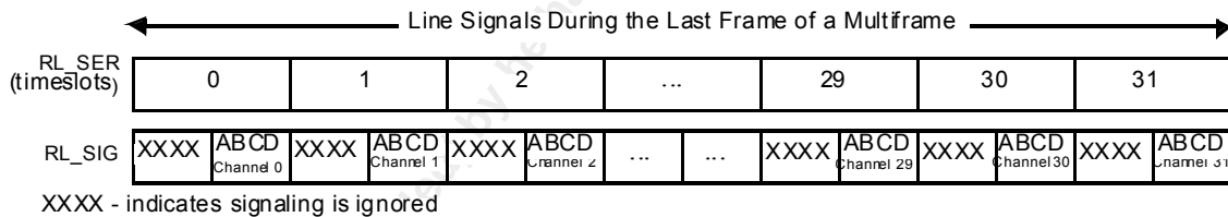
Figure 69 Capture of E1 Signaling Bits
