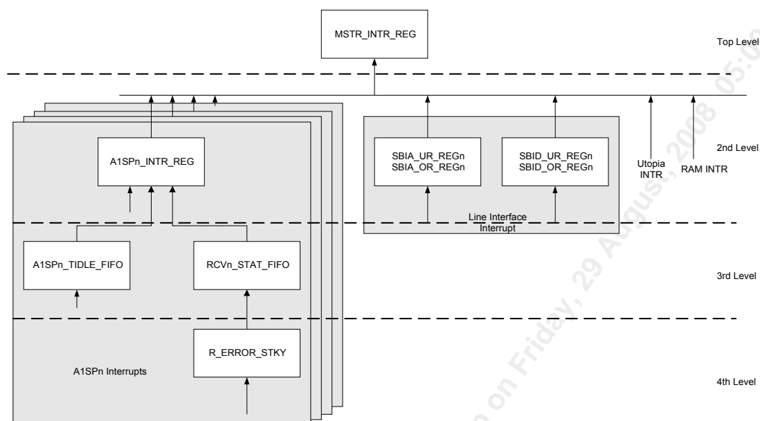
Figure 64 Interrupt Hierarchy
