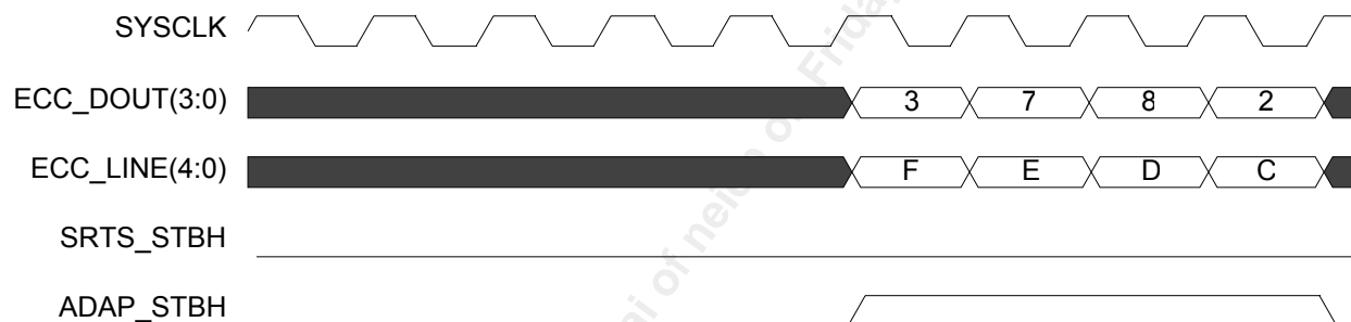
Figure 109 Channel Status Functional Timing
