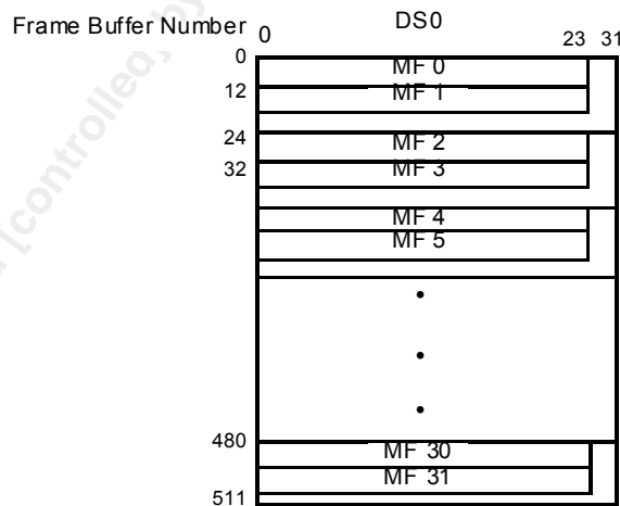
Figure 36 T1 SF SDF-MF Format of the R_DATA_BUFFER
