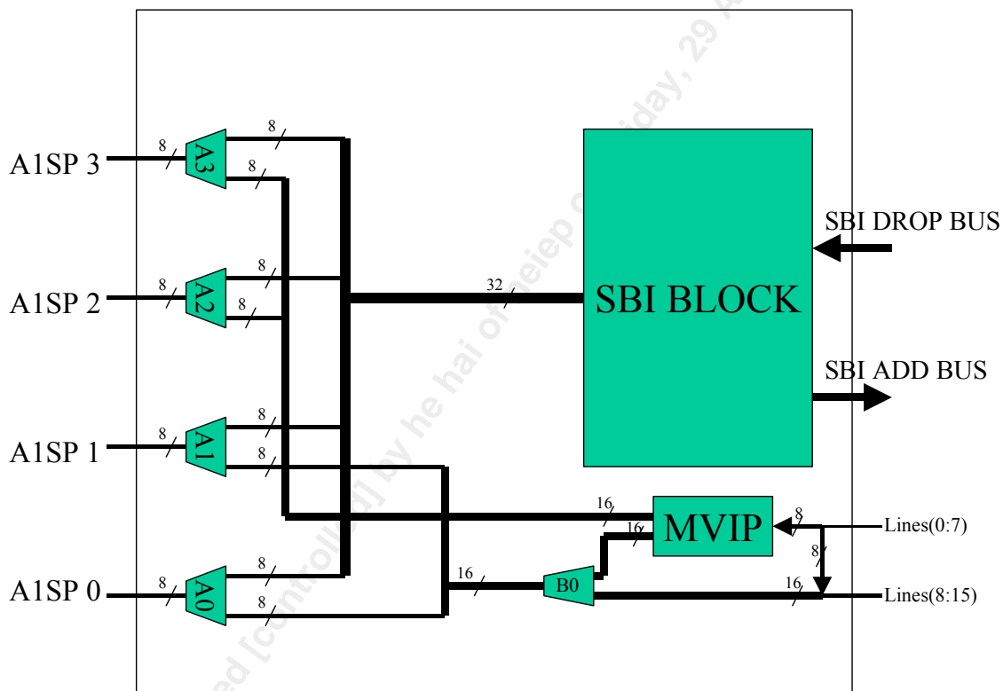
Figure 66 Line Interface Block Architecture
