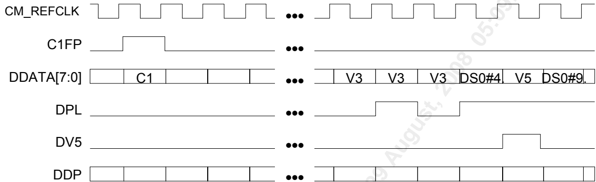
Figure 122 SBI DROP Bus T1/E1 Functional Timing
