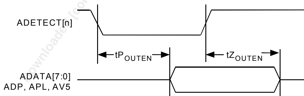
Figure 141 SBI ADD BUS Collision Avoidance Timing
