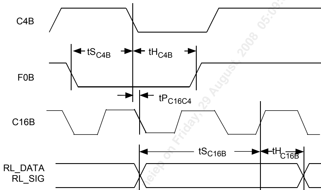
Figure 142 H-MVIP Sink Data & Frame Pulse Timing
