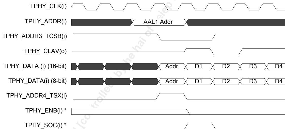
Figure 102 SNK_INTF Start-of-Transfer (Any-PHY PHY Mode)
