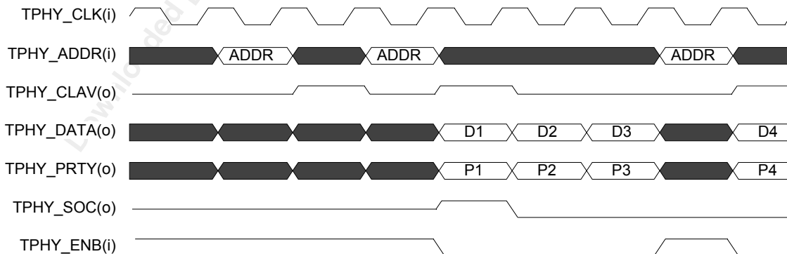
Figure 97 SNK_INTF Start-of-Transfer Utopia 2 (Single Address PHY Mode)
