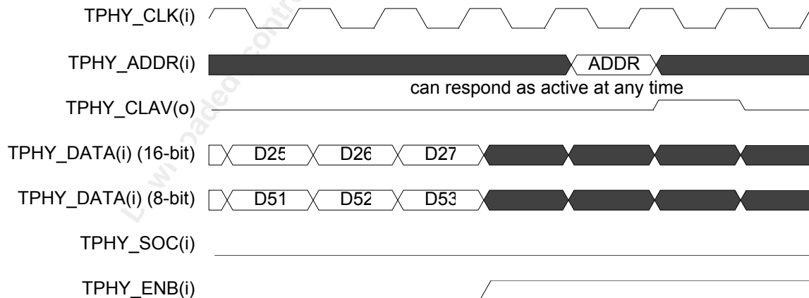
Figure 99 SNK_INTF End-of-Transfer Utopia 2 (Single Address PHY Mode)
