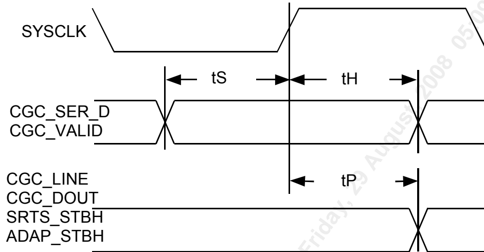
Figure 132 External Clock Generation Control Interface Timing
