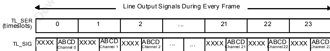
Figure 48 Output of T1 Signaling Bits (SHIFT_CAS=0)
