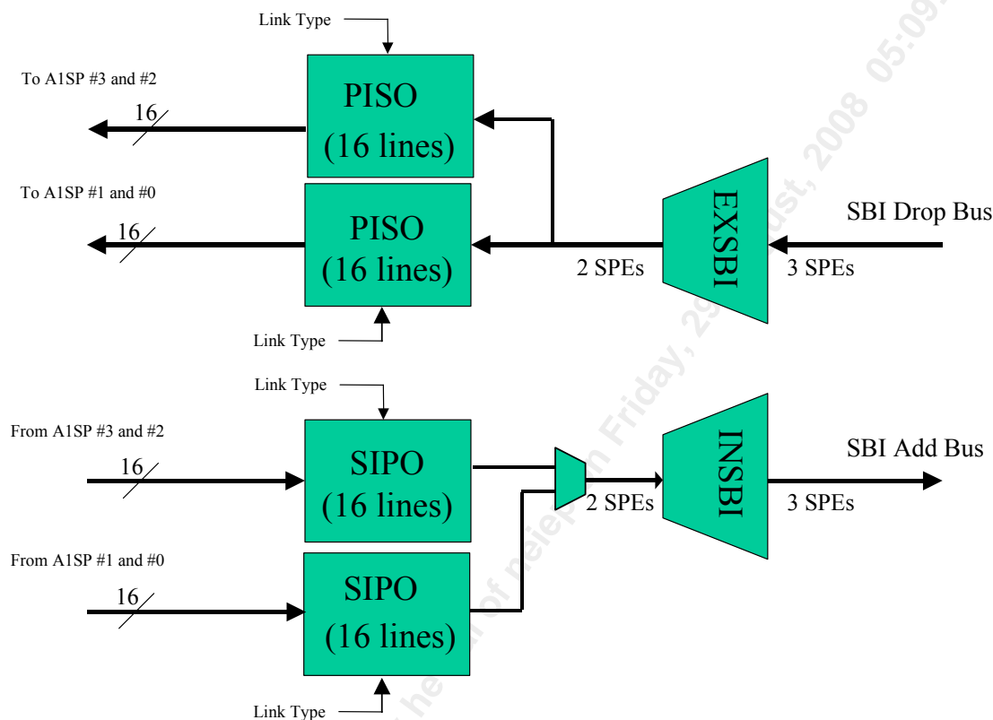
Figure 74 SBI Block Architecture
