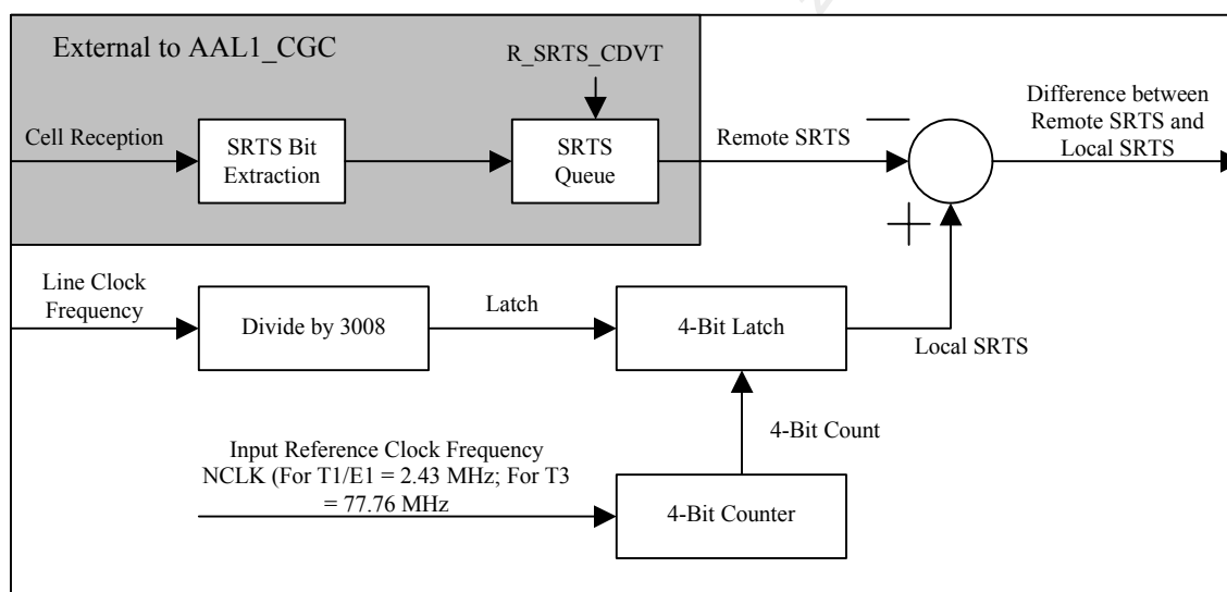
Figure 56 Receive Side SRTS Support
