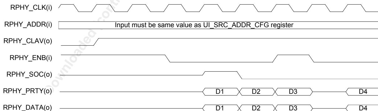
Figure 88 UI_SRC_INTF Start-of-Transfer Timing (Utopia 1 PHY Mode)
