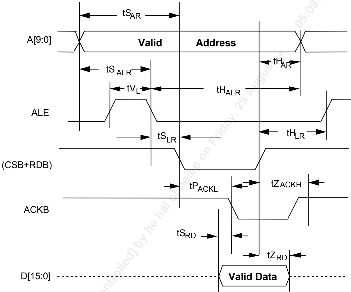
Figure 130 Microprocessor Interface Read Timing
