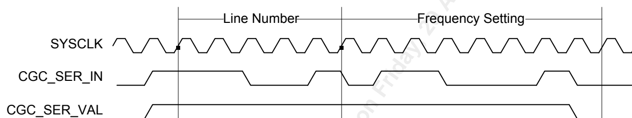
Figure 55 Ext Freq Select Functional Timing
