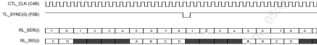
Figure 114 MVIP-90 Receive Functional Timing
