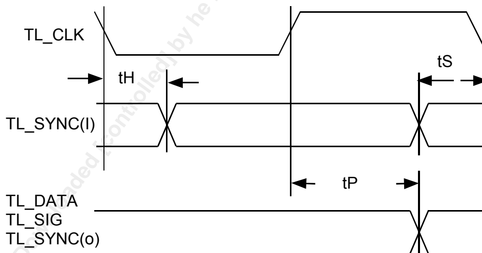
Figure 136 Transmit Low Speed Interface Timing
