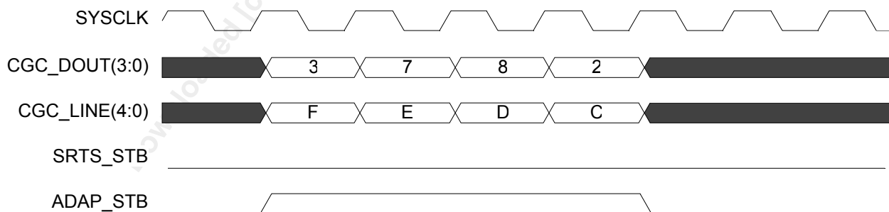
Figure 53 Channel Status Functional Timing
