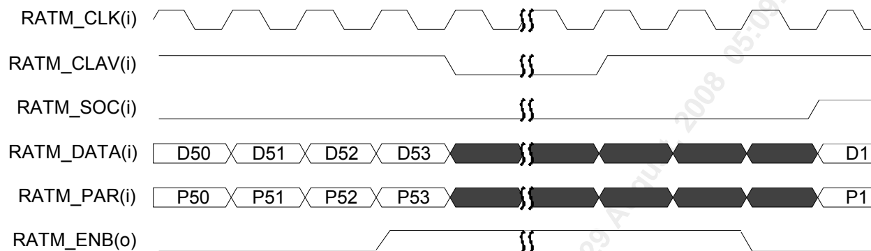
Figure 95 SNK_INTF End-of-Transfer Timing (Utopia 1 ATM Mode)
