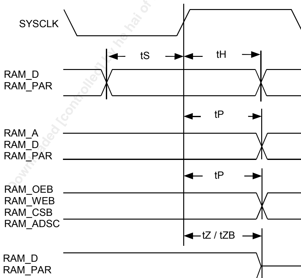
Figure 133 RAM Interface Timing
