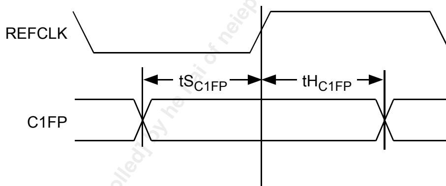
Figure 138 SBI Frame Pulse Timing
