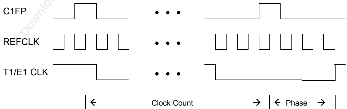
Figure 72 T1/E1 Link Rate Information
