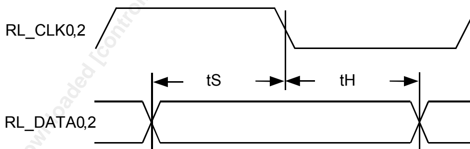
Figure 145 Receive High Speed Interface Timing
