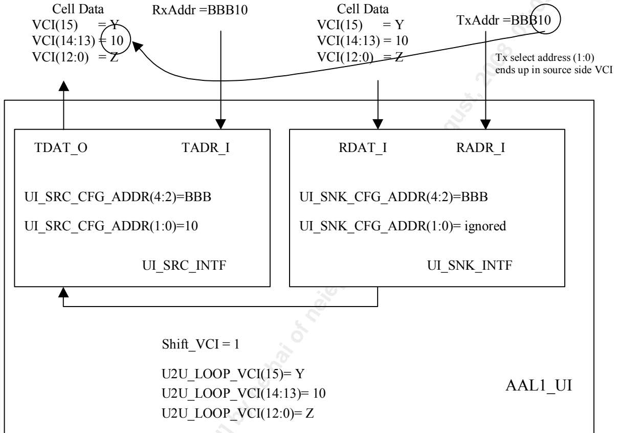
Figure 77 Utopia-2 Multi-Address Mode with VCI Based Loopback
