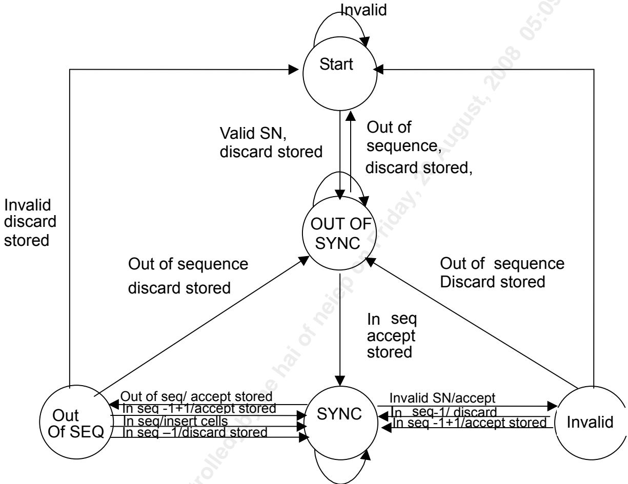
Figure 33 Robust SN Algorithm
