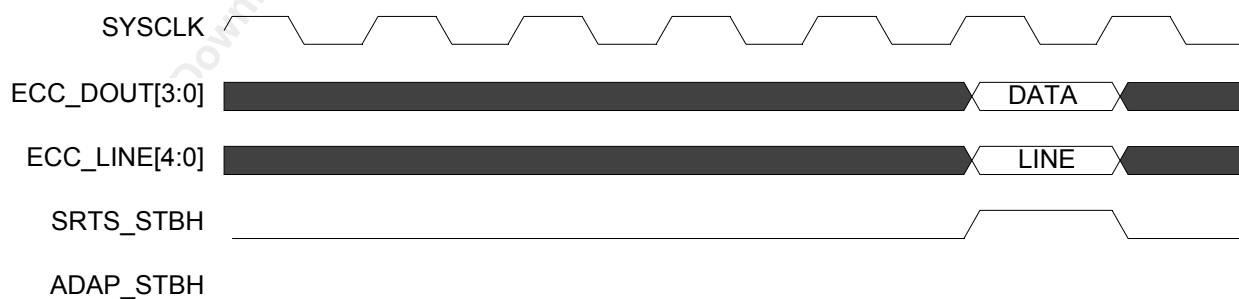
Figure 108 SRTS Data
