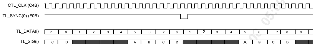
Figure 117 MVIP-90 Transmit Functional Timing
