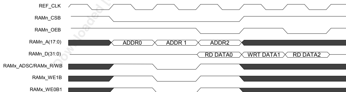
Figure 85 Pipelined ZBT SSRAM
