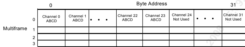
Figure 20 SDF-MF T1 ESF Format of the T_SIGNALING_BUFFER
