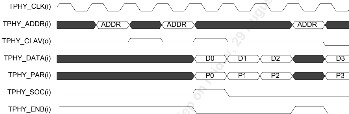
Figure 100 SNK_INTF Start-of-Transfer Utopia 2 (Multi-Address PHY Mode)
