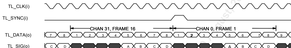
Figure 116 Transmit Line Side E1 Timing(TL_CLK = 2.048 MHz)
