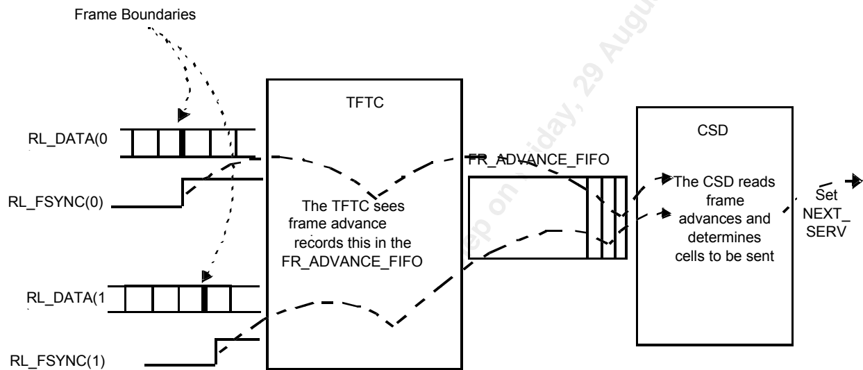
Figure 27 Frame Advance FIFO Operation
