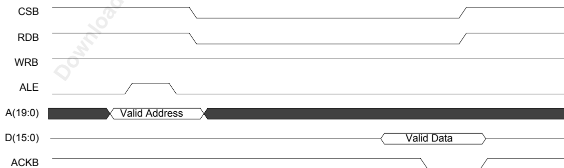
Figure 107 Microprocessor Read Access with ALE
