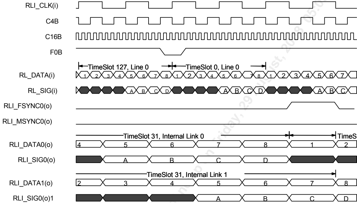
Figure 118 Receive H-MVIP Timing, Close-Up View
