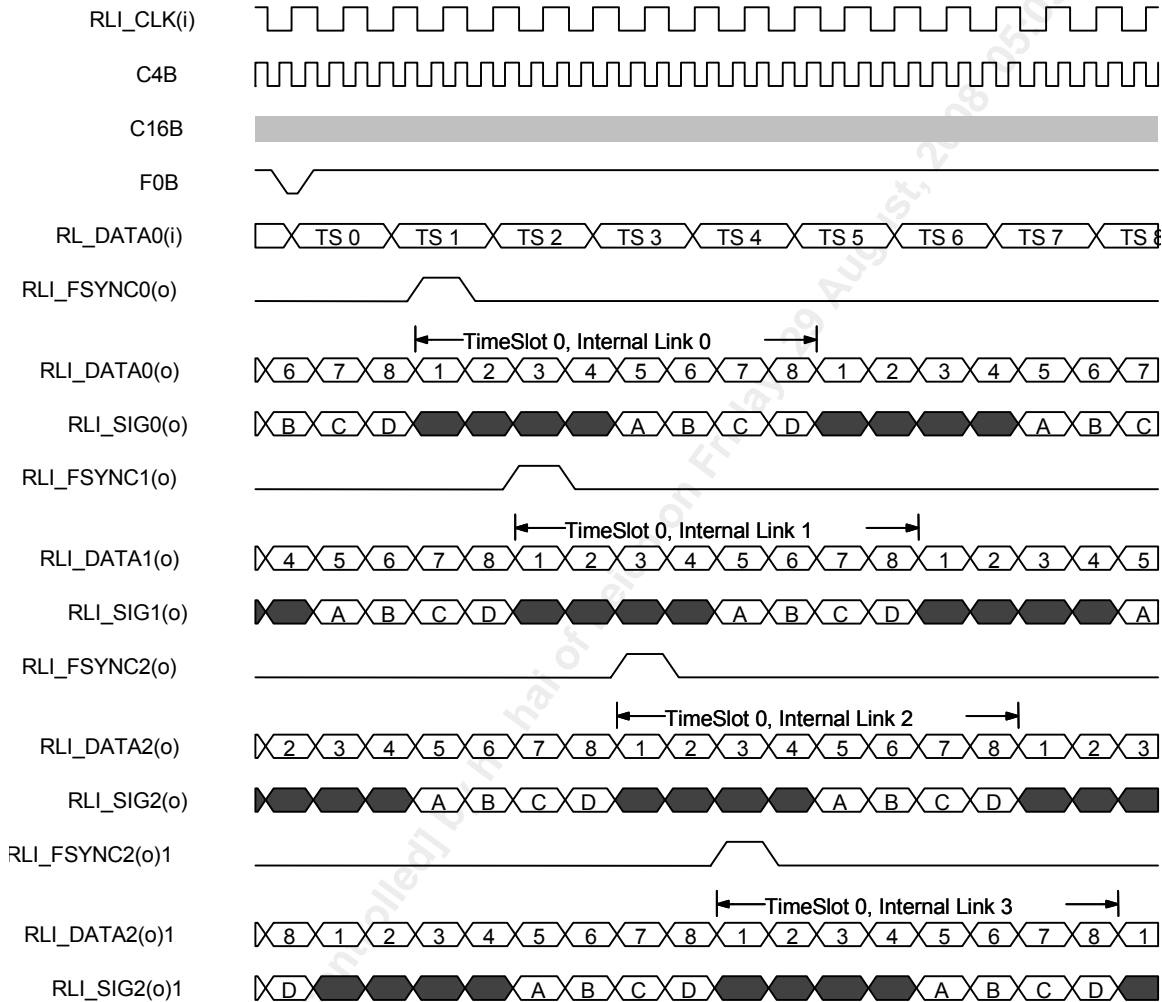
Figure 119 Receive H-MVIP Timing, Expanded View
