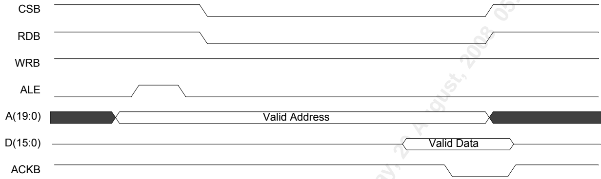
Figure 106 Microprocessor Write Access with ALE
