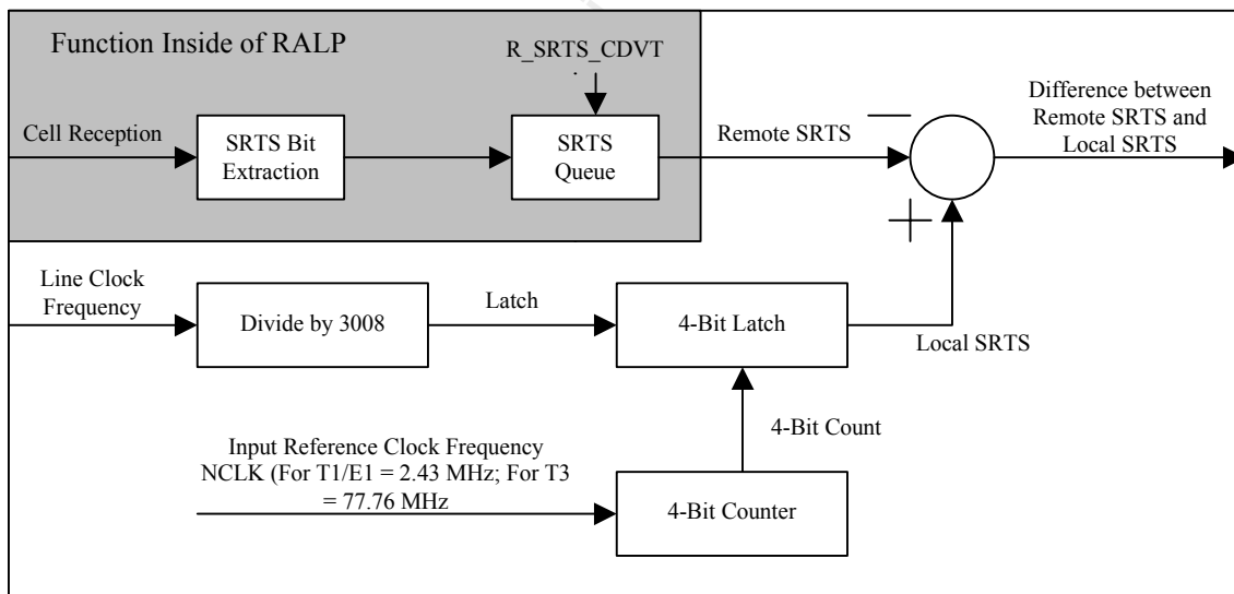
Figure 51 Receive Side SRTS Support
