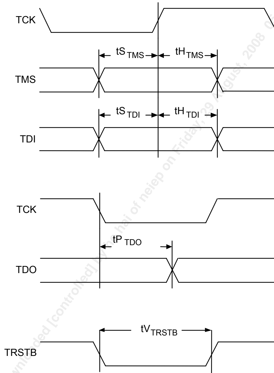
Figure 146 JTAG Port Interface Timing
