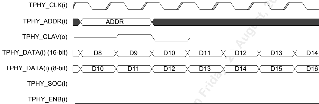
Figure 98 SNK_INTF CLAV Disable Utopia 2 (Single-Address PHY Mode)
