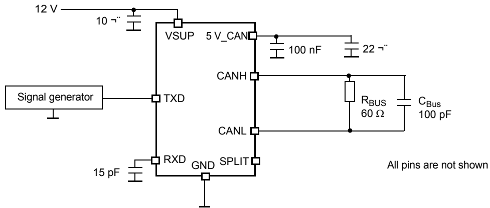
Figure 19. Test Circuit for CAN Timing Characteristics
