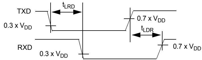
Figure 17. CAN Signal Propagation Loop Delay TXD to RXD
