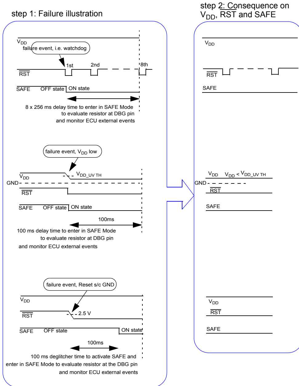
Figure 33. SAFE Mode A Behavior Illustration
