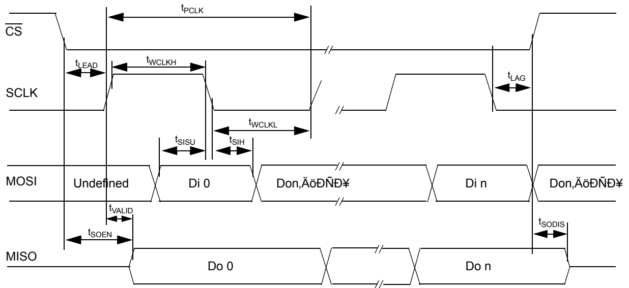
Figure 16. SPI Timings
