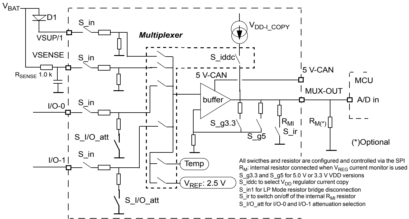
Figure 24. Analog Multiplexer Block Diagram
