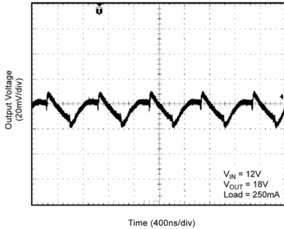
Ripple Waveform
