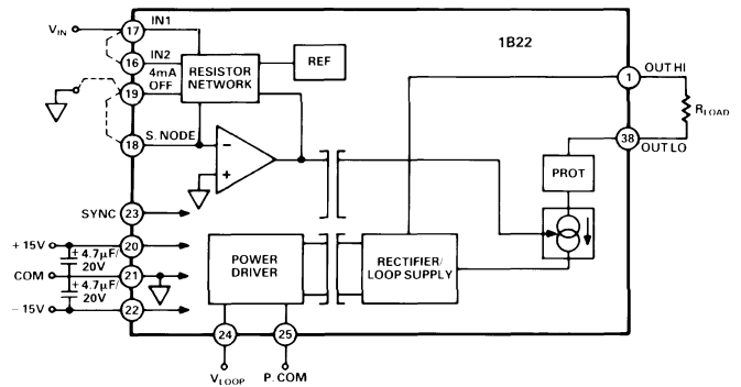
Figure 2. Basic Interconnections
