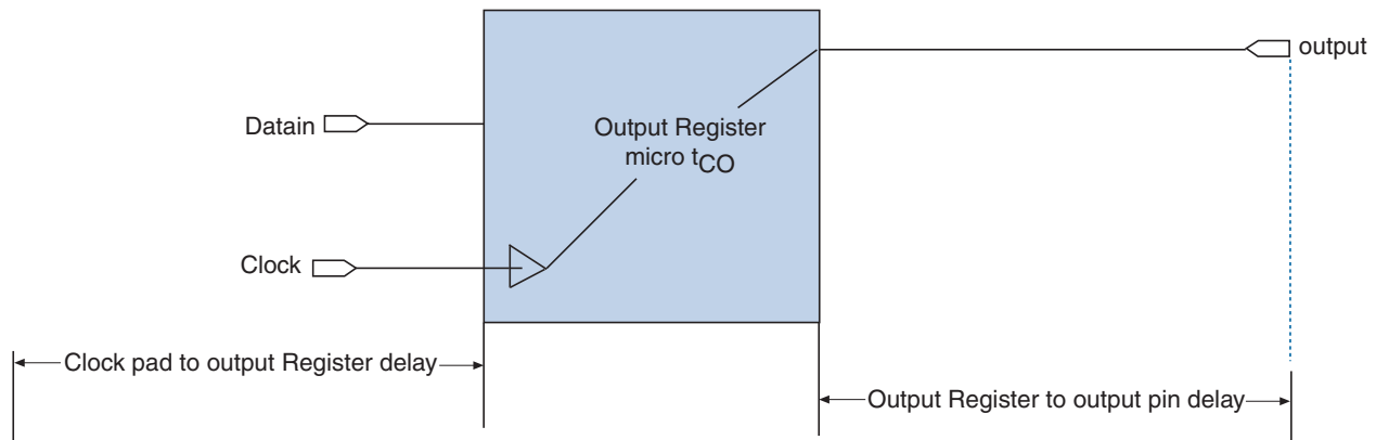
Figure 1–2. Output Register Clock to Output Timing Diagram
