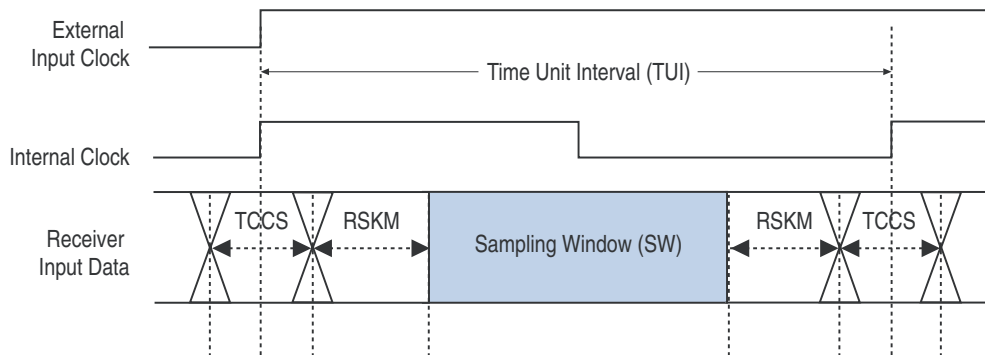
Figure 8–23. High-Speed I/O Timing Diagram
