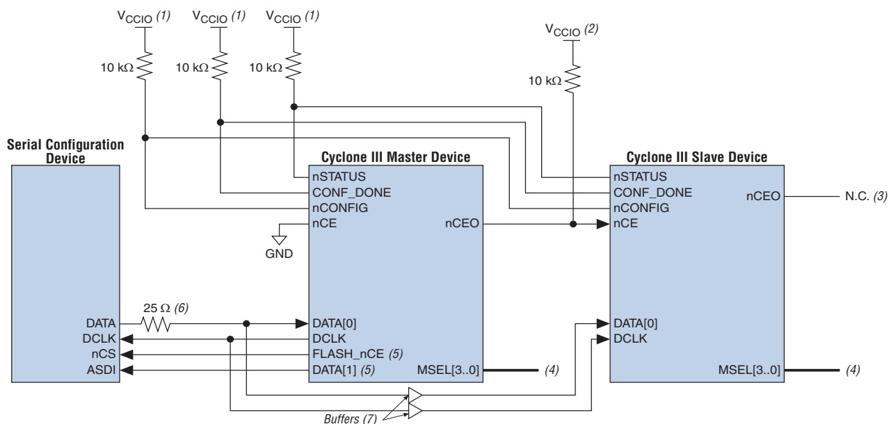
Figure 10–4. Multi-Device AS Configuration
