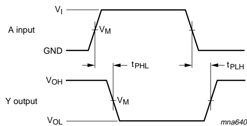
Fig 7. The input A to output Y propagation delays
