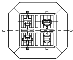
VIEW "A"
