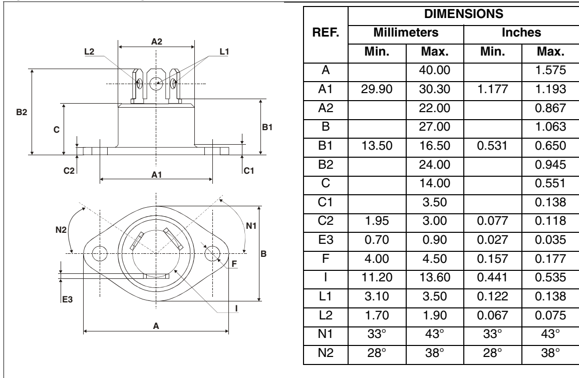
Figure 12: RD91 Package Mechanical Data
