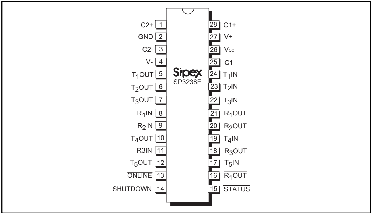
Figure 4. SP3238E Pinout Configuration
