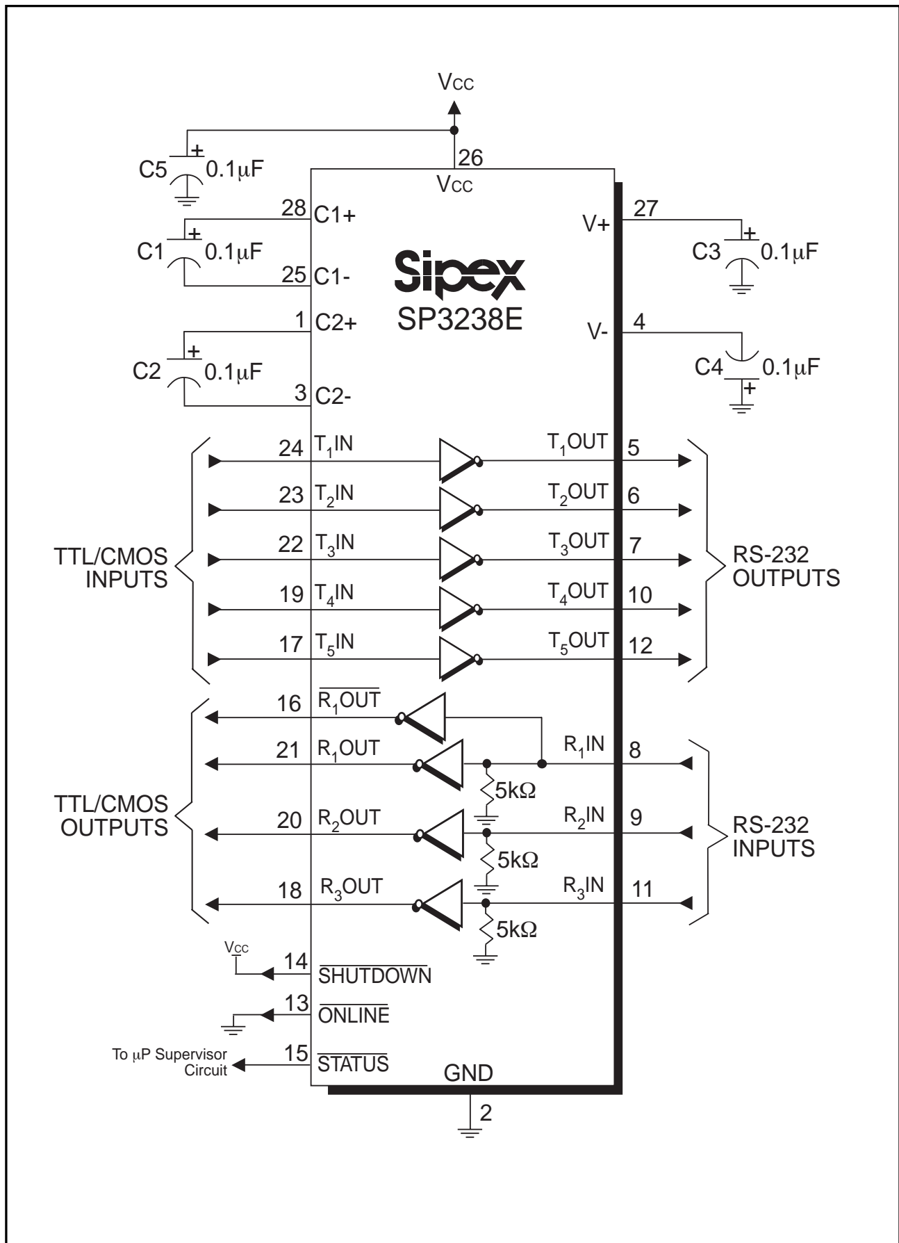
Figure 5. SP3238E Typical Operating Circuit
