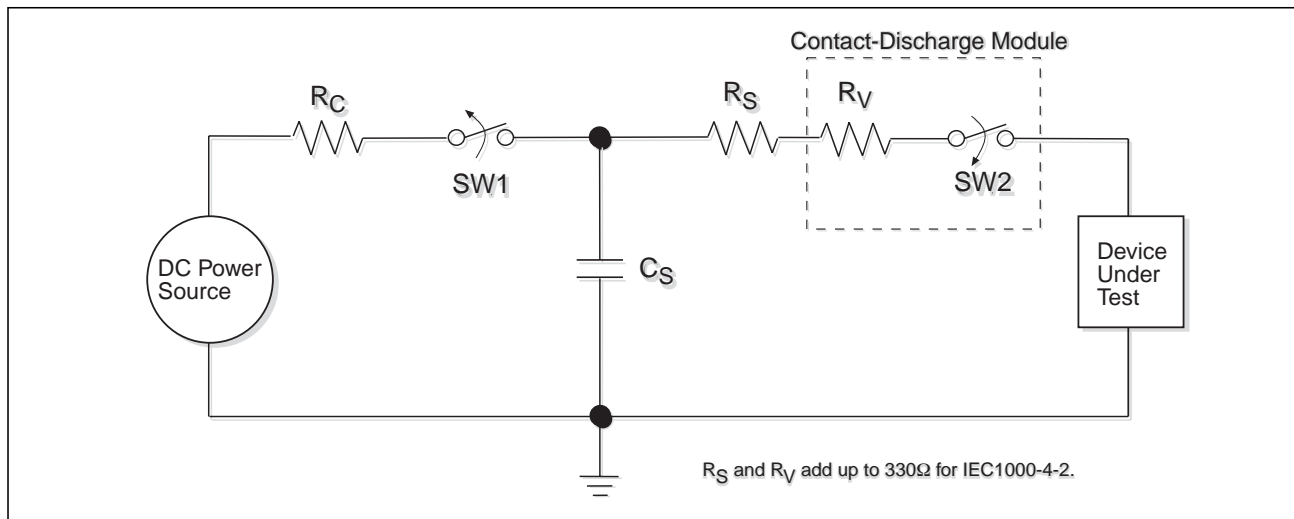
Figure 20. ESD Test Circuit for IEC1000-4-2
