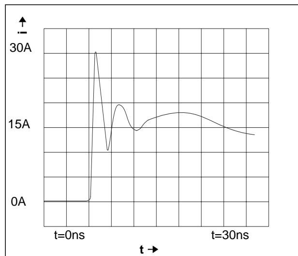
Figure 21. ESD Test Waveform for IEC1000-4-2
