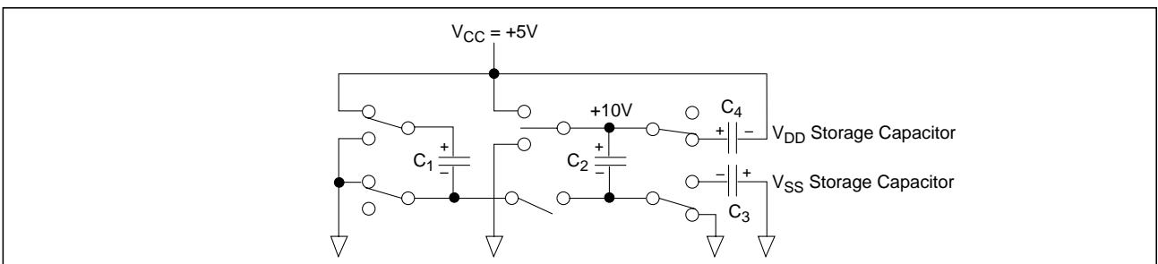
Figure 15. Charge Pump — Phase 4
