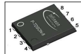
P-TDSON-8
