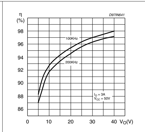
Figure 26. Efficiency vs. output voltage (see Figure 4)
