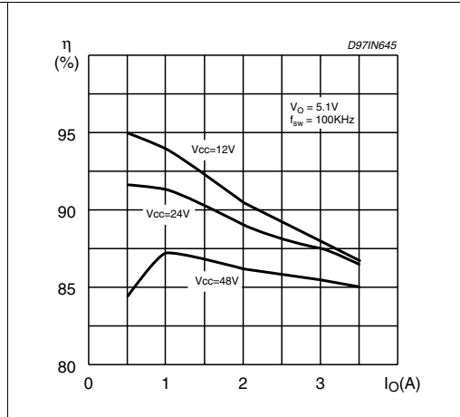
Figure 30. Efficiency vs. output current (see Figure 8)
