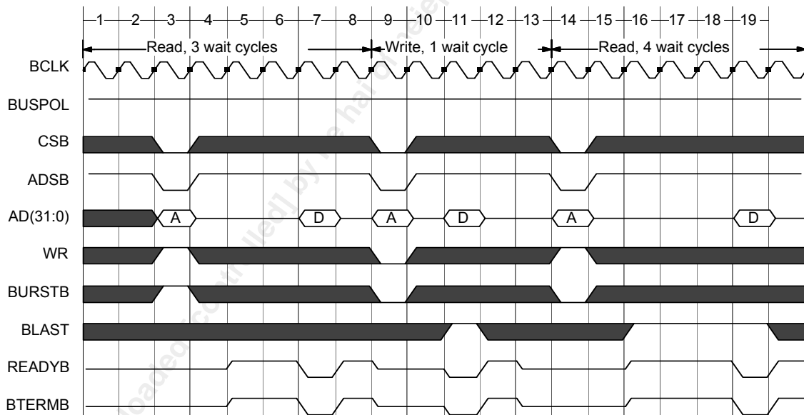
Figure 33 - Single Word Read and Write to Non-burstable Address Space
