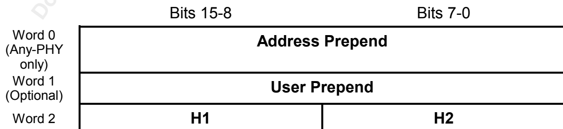
Figure 3 - 16bit Receive Cell Transfer Format
