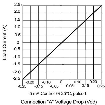
Figure 3. Linearity Characteristics
