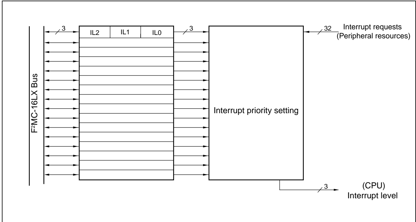
(2) Block Diagram
