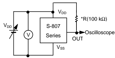
(1) Detection voltage
