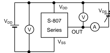
(b) Pch transistor current
