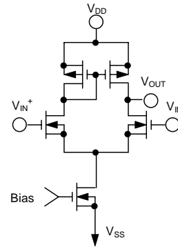
Figure 15 Comparator
