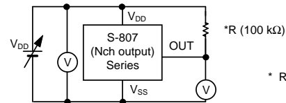
(4) Min. operating voltage
