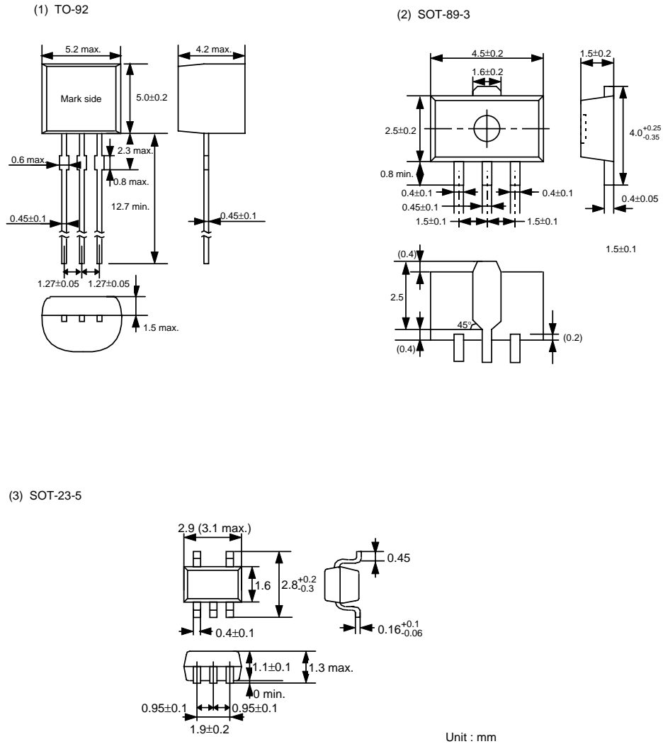
Figure 16 Dimensions
