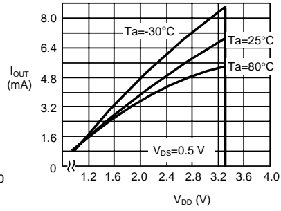
(ii) V_{DD} - I_{OUT}
