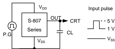
(b) CMOS output products
