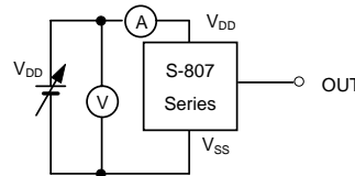
(2) Current consumption
