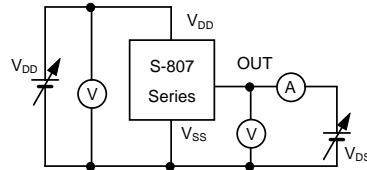
(a) Nch transistor current
