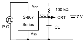
(a) Nch open-drain output products
